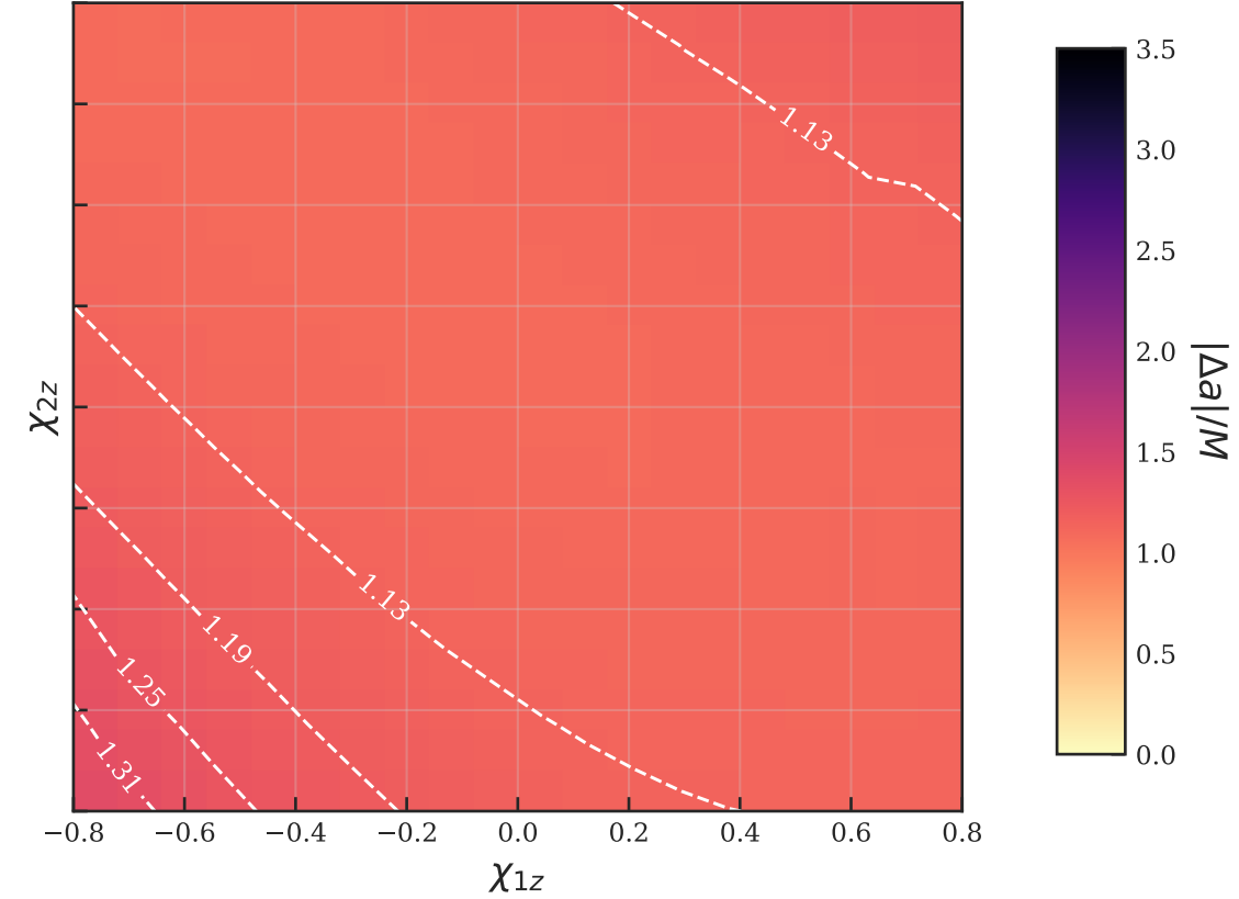
Taylor 2PN
