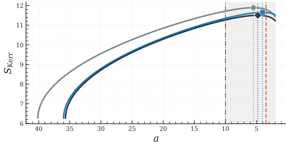
Padé extrapolation
