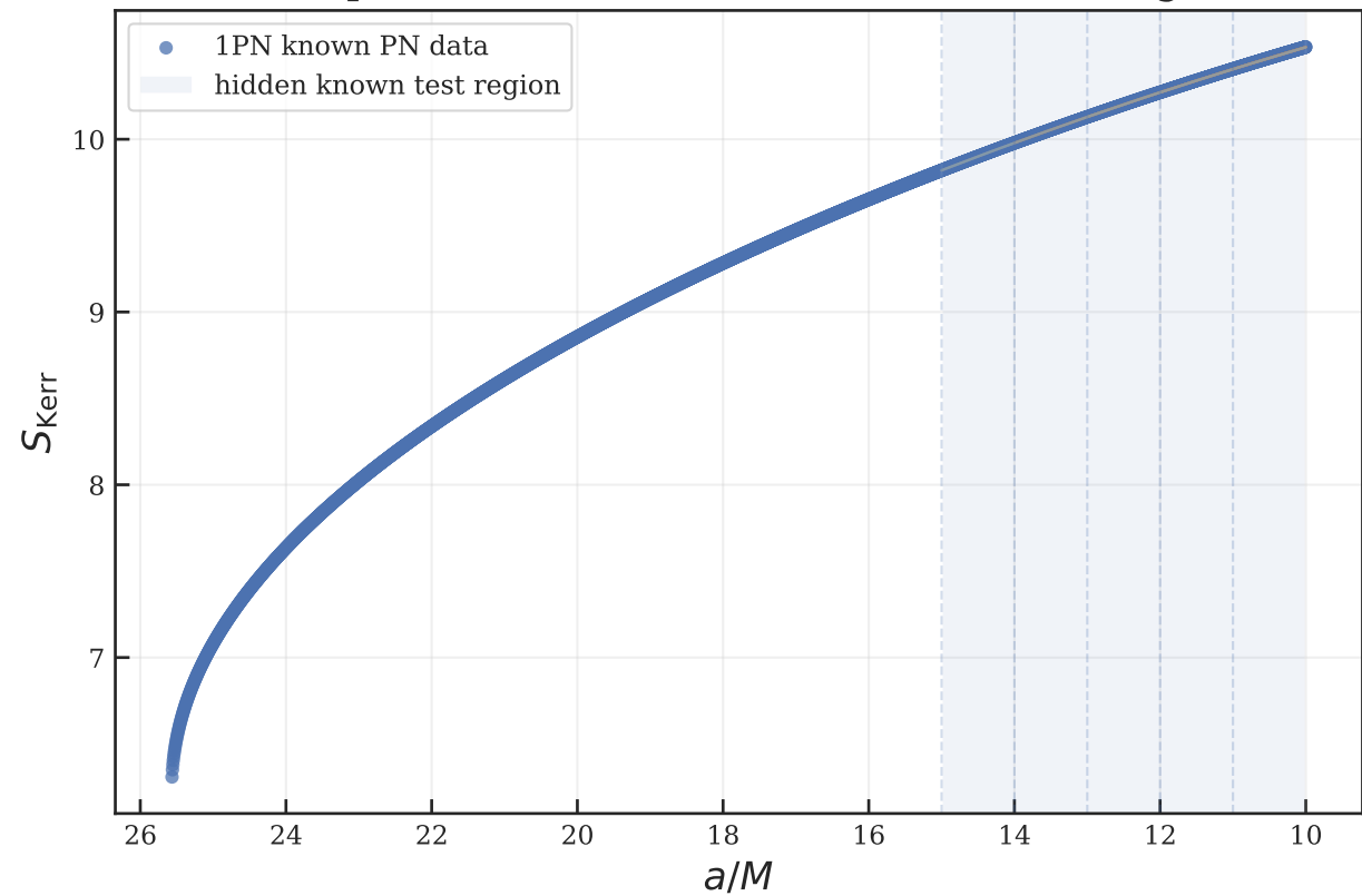
Padé predictions tested inside known PN region
