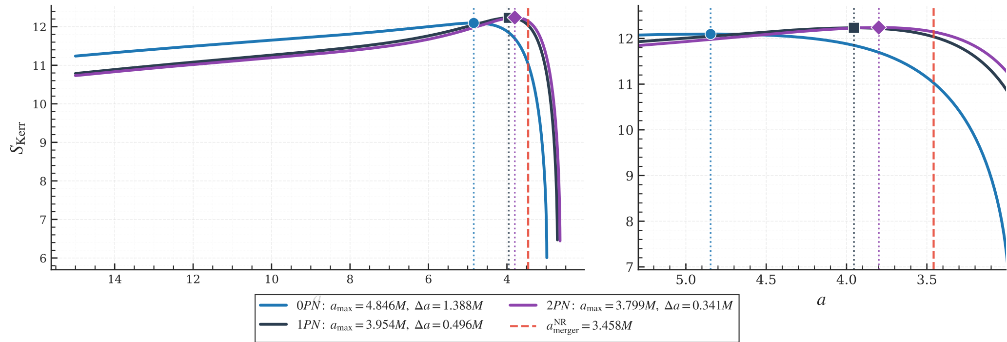
Taylor extrapolation
