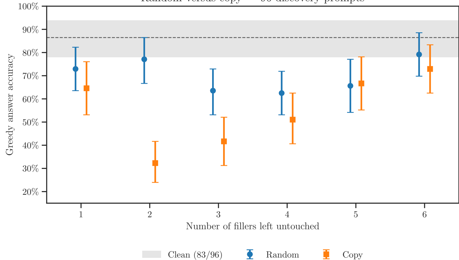
Random versus copy — 96 discovery prompts
