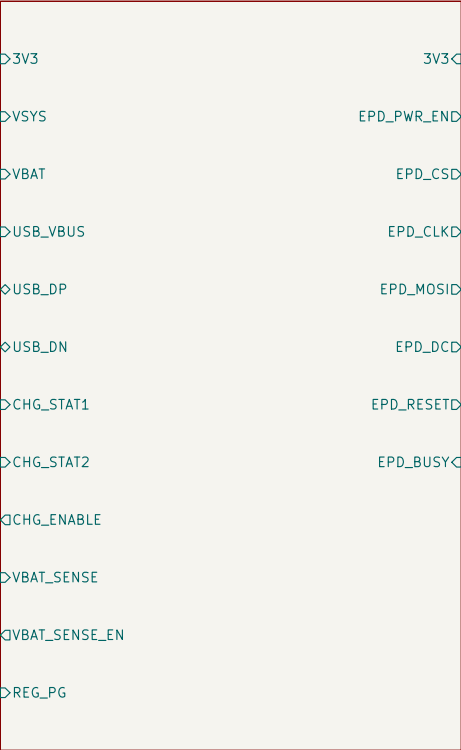
Controller and user I/O
