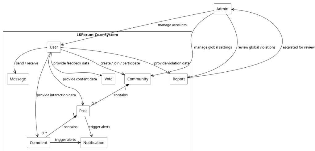
Figure 2.1: Domain Model Diagram
