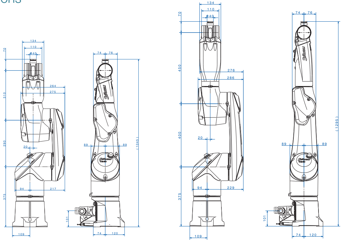
Mounting (not for vertical cable outlet option)
