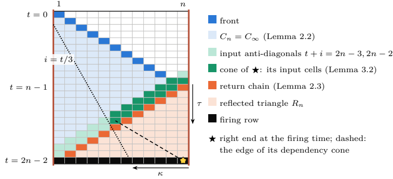
Figure 1: The line of length n = 12 (time downwards; colours show regions, not states). R_n is computed from the two input anti-diagonals (Lemma 3.1); the firing of the right end (★) depends only on the dark input cells (Lemma 3.2), which end where the line i = t/3 crosses the input anti-diagonals (Theorem 3.4).
