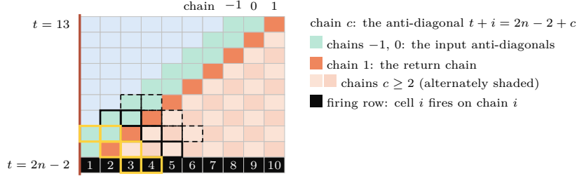
Figure 2: The lower left corner of the line of length n = 12 (time downwards; colours show regions, not states). Outlined: three slices for s = 2 (dashed y = 4 , solid y = 3 , yellow y = s ), each made of the input cells u_{-1}(y), u_0(y) (upper left) and the band cells u_1(y), \dots, u_4(y) ; slice y is computed from slice y + 1 (the map \Gamma in the proof of Lemma 4.1), and slice s contains the firing cells 2s - 1 and 2s .
