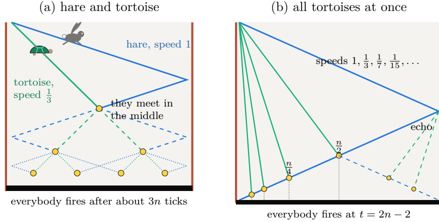
Figure 7: Space-time sketches of two classical constructions (time runs downwards; borders in red). (a) Halving: the hare (speed 1) and the tortoise (speed \frac{1}{3} ) meet in the middle, and the construction is repeated in both halves, here for n = 17 . (b) Minimal time, n = 33 : signals of speeds 1/(2^j - 1) meet the reflected signal at n/2, n/4, n/8, \dots ; each piece is synchronized from one of its ends, as shown with dashes for the right half, and all pieces fire at t = 2n - 2 = 64 .
