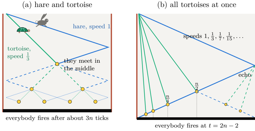
Figure 4: Space-time sketches of two classical constructions (time runs downwards; walls in red). (a) Halving: the hare (speed 1) and the tortoise (speed 1/3 ) meet in the middle; the construction is repeated in both halves, here for n = 17 . (b) Minimal time, n = 33 : signals of speeds 1/(2^j - 1) meet the echo at n/2, n/4, n/8, \dots ; each piece is synchronized by a general at one of its ends, as shown with dashes for the right half, and all pieces fire at t = 2n - 2 = 64 .
