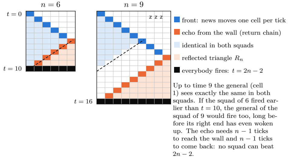
Figure 3: Space-time diagrams (time runs downwards, one square per cell and tick) of squads of 6 and of 9 soldiers, coloured by what each cell can know. On the cells with t + i \leq 10 (light blue, bounded by the dashed anti-diagonal) the two diagrams are equal cell by cell, for every rule (Lemma 2.2); the right border can only act in the reflected triangle, below the echo. The colours show regions, not states.
