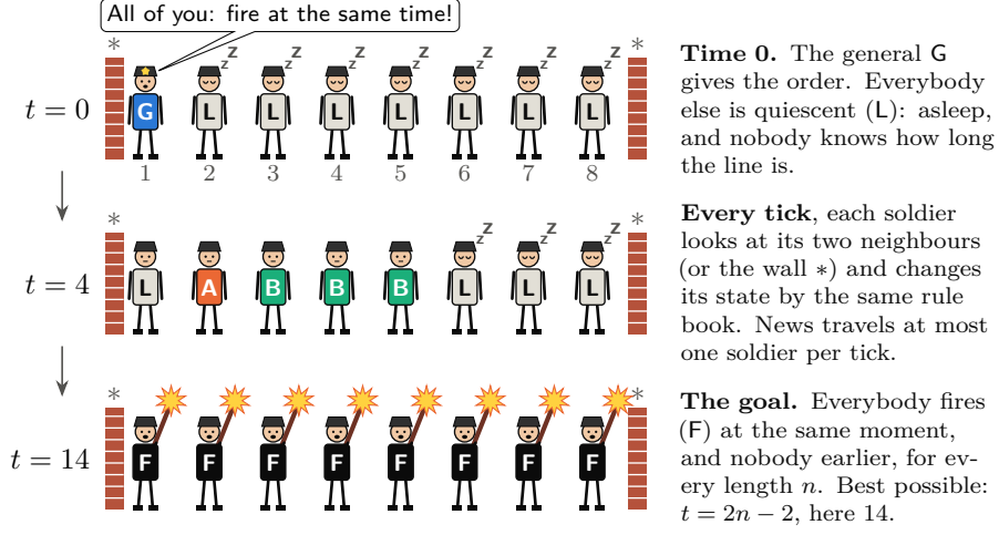
Figure 1: A squad of n = 8 . Top: at time 0 the general (G) gives the order and everybody else is quiescent (L). Middle: at time 4 the news has reached cell 5, and cells 6 to 8 are still asleep. Bottom: at time 2n - 2 = 14 all soldiers fire together. The three rows are the configurations of the rule \delta_{14} on the line of length 8 at the times 0, 4 and 14.
