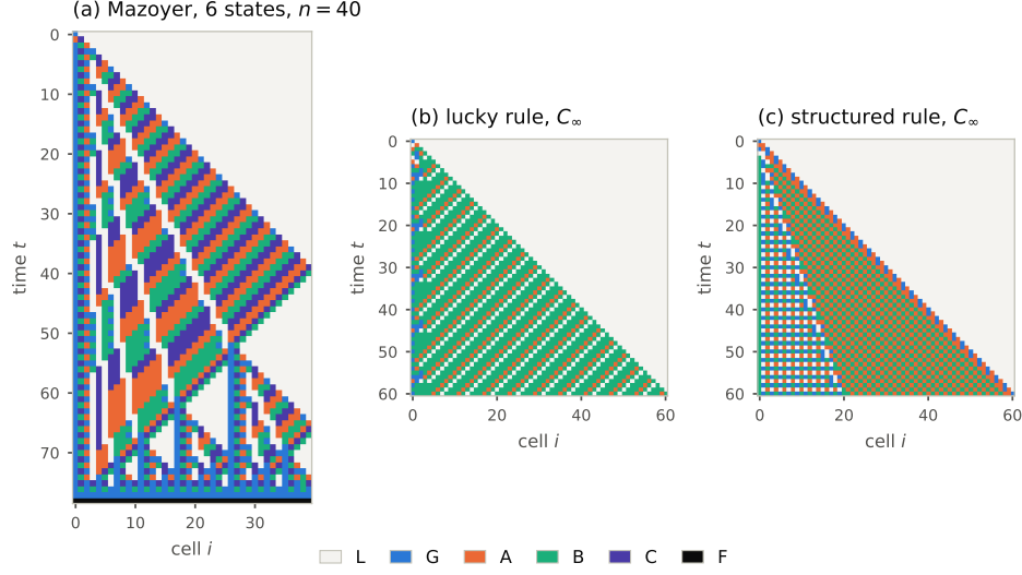
Figure 7: Space-time diagrams, time downwards. (a) Mazoyer’s six-state solution on n = 40 cells; the last row is the firing row. (b) Half-line of a five-state rule that synchronizes the lengths 2, \dots, 9 and 20 but violates the pumping lemma: its background is periodic. (c) Half-line of a five-state rule found under the pumping constraints: the boundary between the checkered region and the diagonal background has slope 1/3 .
