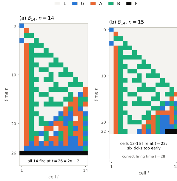
Figure 6: The five-state rule \delta_{14} (Table A.7) on squads of 14 and 15 soldiers (time runs downwards, one square per cell and tick, coloured by state). (a) All 14 cells fire at t = 26 = 2n - 2 . (b) The cells 13, 14 and 15 fire at t = 22 , before the correct firing time t = 28 . Computed by direct simulation ( fsspcheck.c ).
