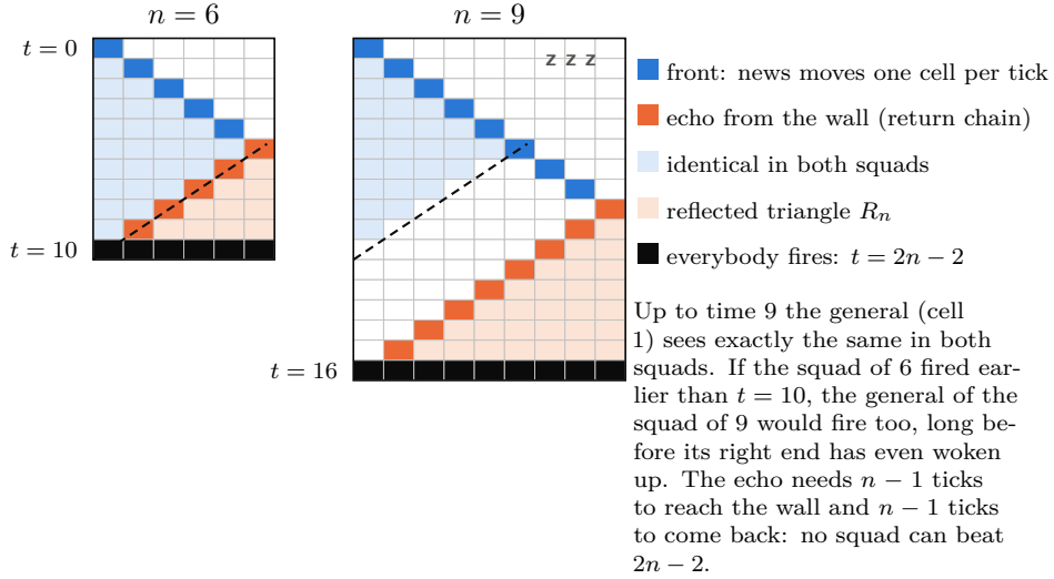
Figure 4: Space-time diagrams (time runs downwards, one square per cell and time step) of the lines of lengths 6 and 9, coloured by what each cell can know. On the cells with t + i \leq 10 (light blue, bounded by the dashed anti-diagonal) the two diagrams coincide for every rule (Lemma 2.2); the right border acts only in the reflected triangle R_n , below the return chain. The colours show regions, not states.
