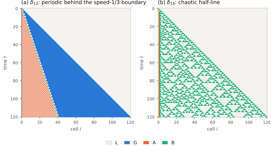
Figure 2: Half-lines of the two frontier architectures (time downwards, 0 \leq t \leq 120 ). (a) The common half-line of \delta_{12} and \delta_{13} : a front and a solid wake of G 's and a checkered region of A 's and L 's behind a boundary of speed 1/3 ; the checkered region is excluded by Lemma 3.5 (Corollary 6.2). (b) The half-line of \delta_{14} , determined by 16 neighbourhoods; its irregular pattern escapes both barriers.
