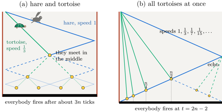
Figure 4: Space-time sketches of two classical constructions (time runs downwards; walls in red). (a) Halving: the hare (speed 1) and the tortoise (speed 1/3 ) meet in the middle; the construction is repeated in both halves, here for n = 17 . (b) Minimal time, n = 33 : signals of speeds 1/(2^j - 1) meet the echo at n/2, n/4, n/8, \dots ; each piece is synchronized by a general at one of its ends, as shown with dashes for the right half, and all pieces fire at t = 2n - 2 = 64 .
