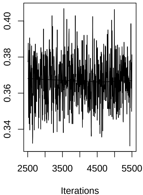
Trace of coefficients
