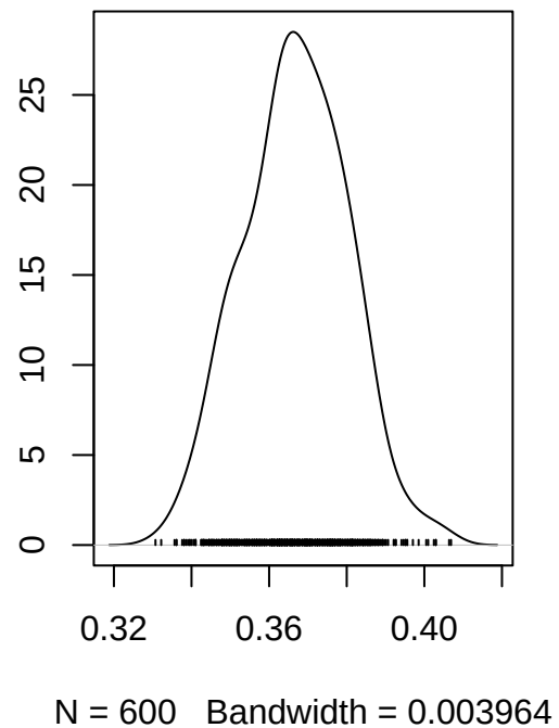
Density of coefficients
