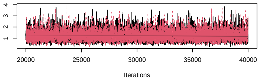
Trace of sigma_sq[2]
