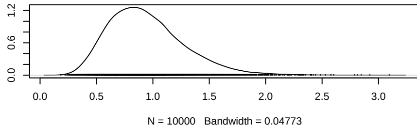
Density of sigma_sq[3]
