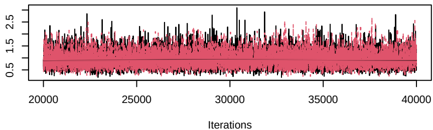
Trace of sigma_sq[3]
