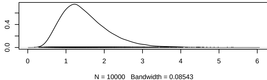
Density of sigma_sq[1]
