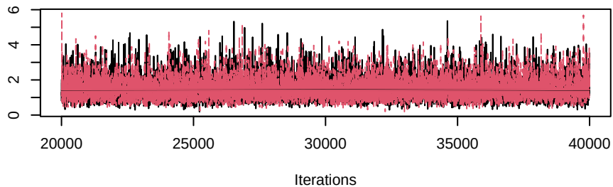
Trace of sigma_sq[1]
