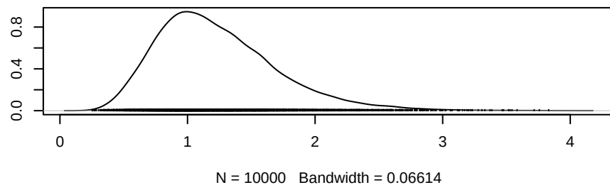
Density of sigma_sq[2]
