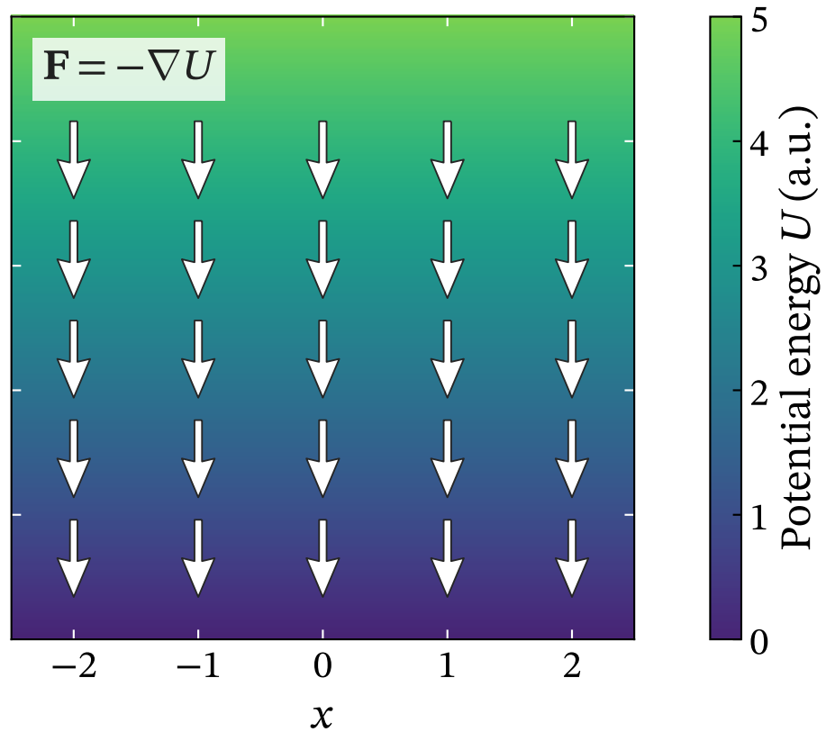
Gravitational force
