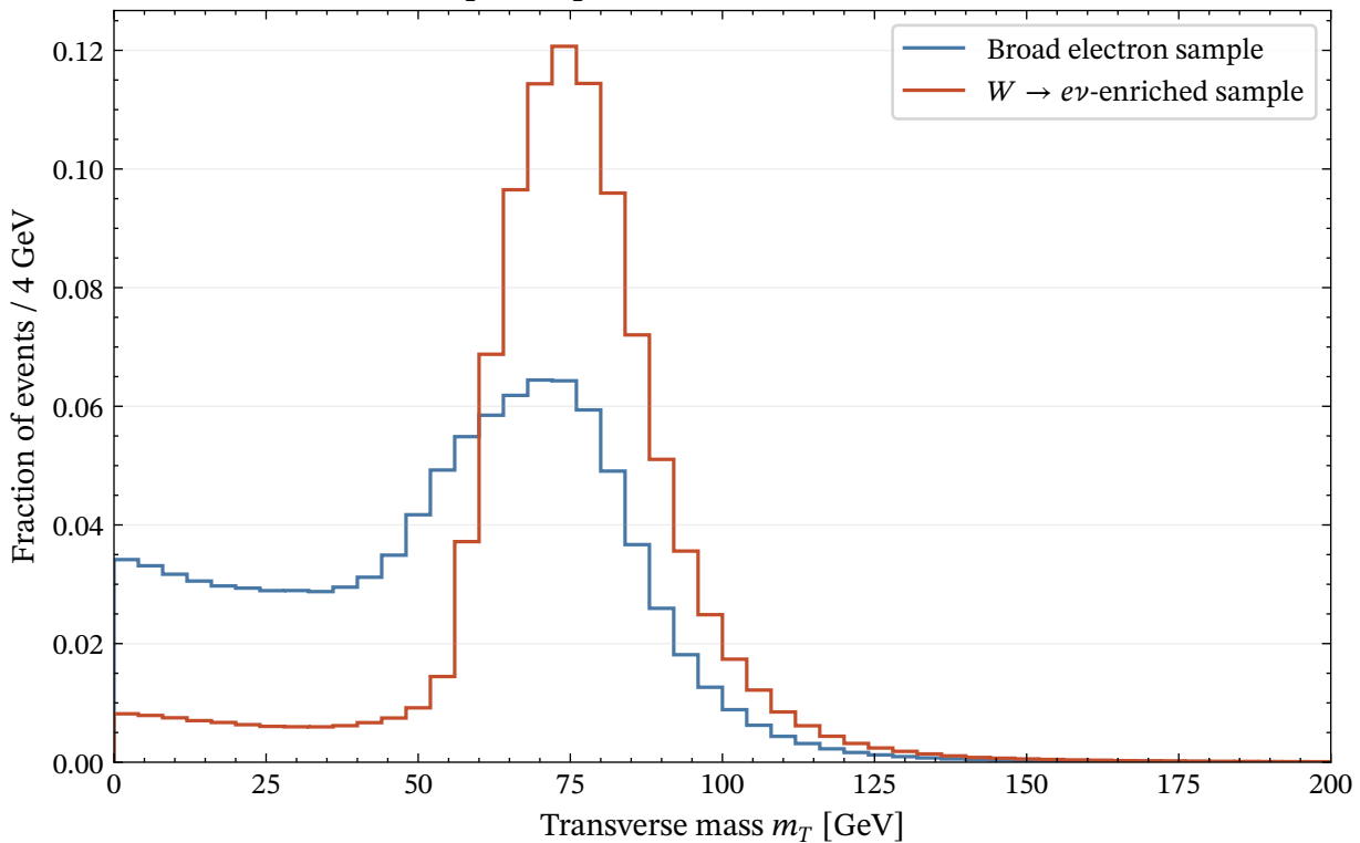
Shape comparison for W \rightarrow e\nu candidates
