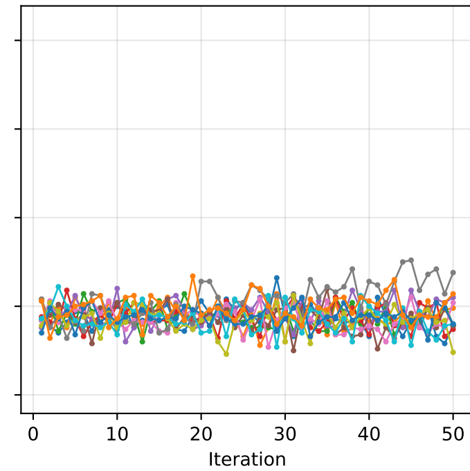
GPHedge
