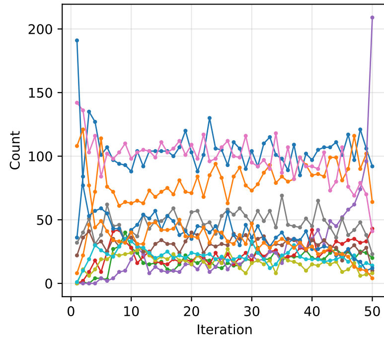
LMABO
