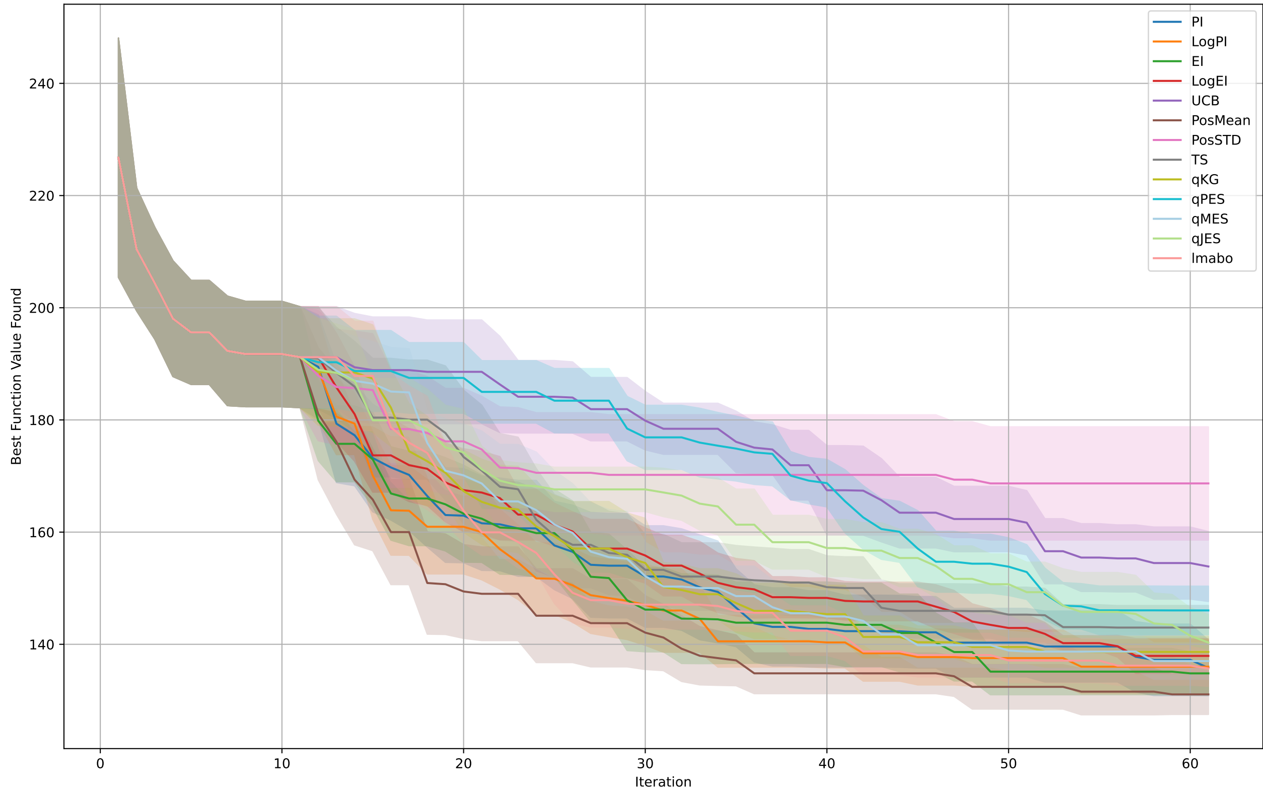
LunacekBiRastrigin
