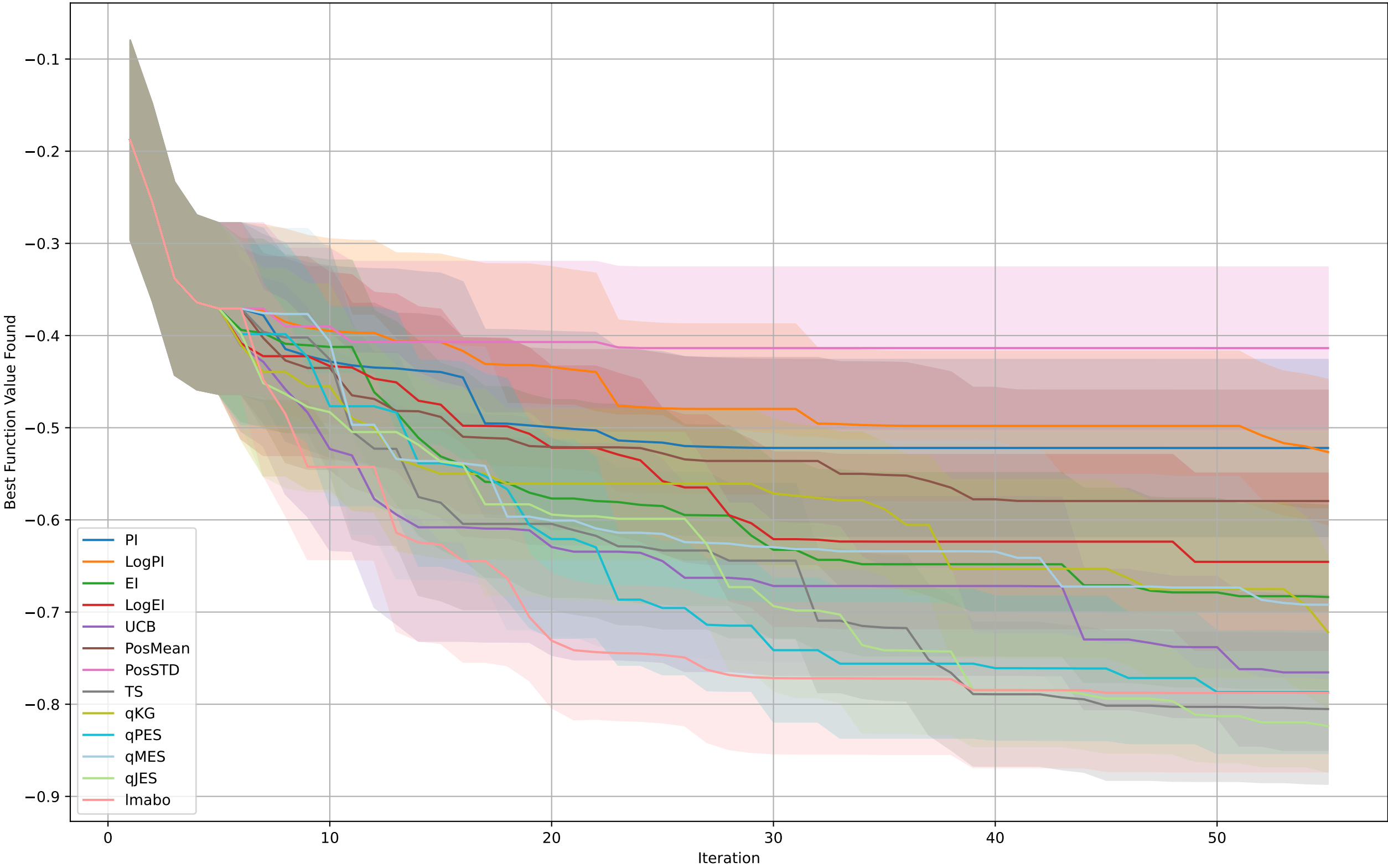
DropWave
