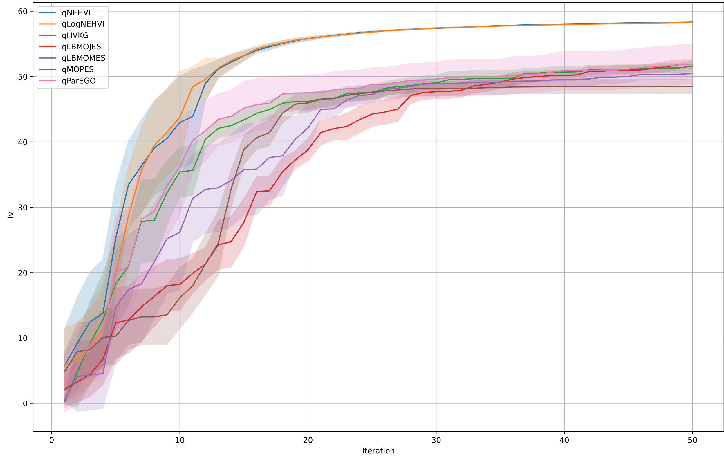
BraninCurrin
