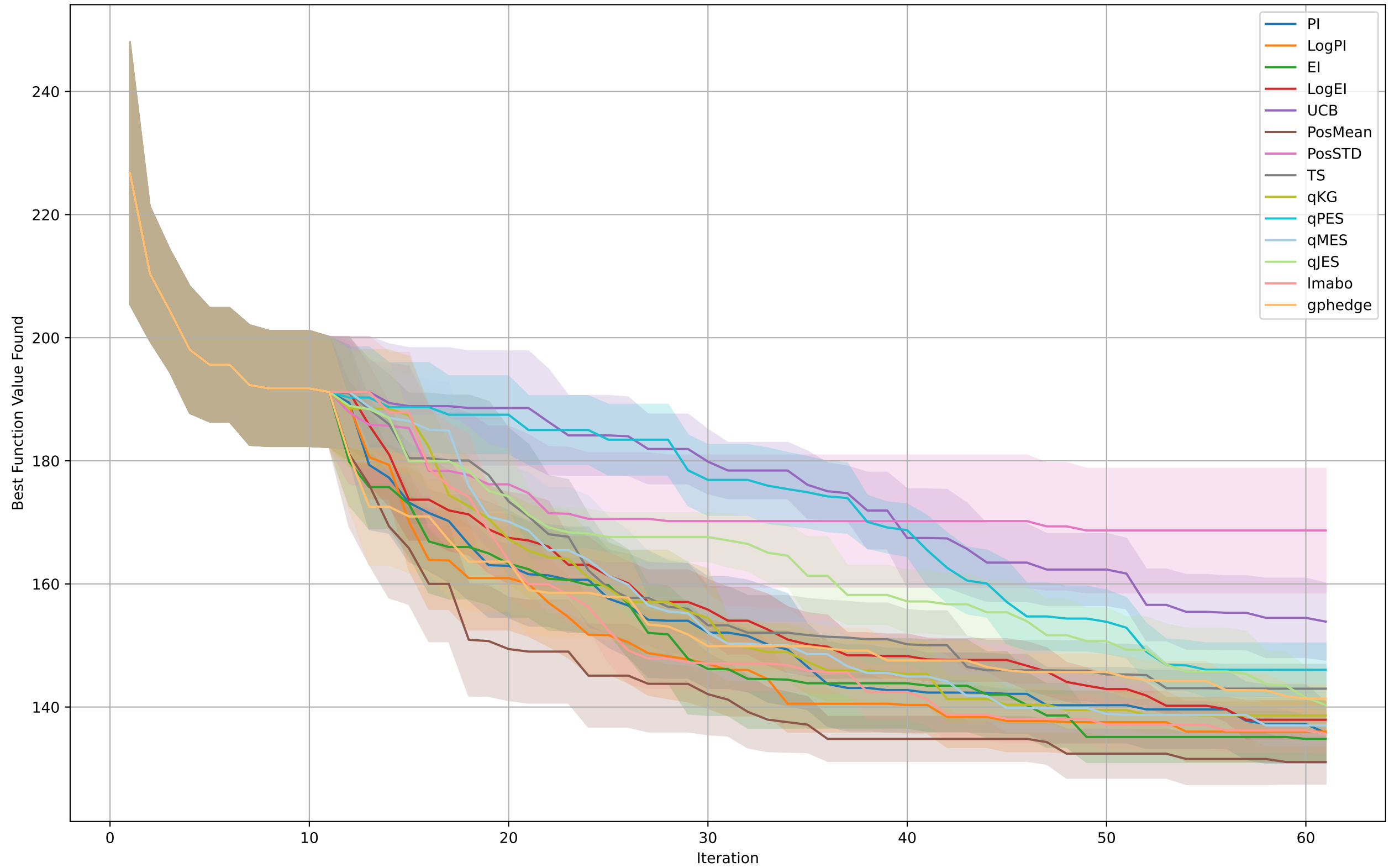
LunacekBiRastrigin
