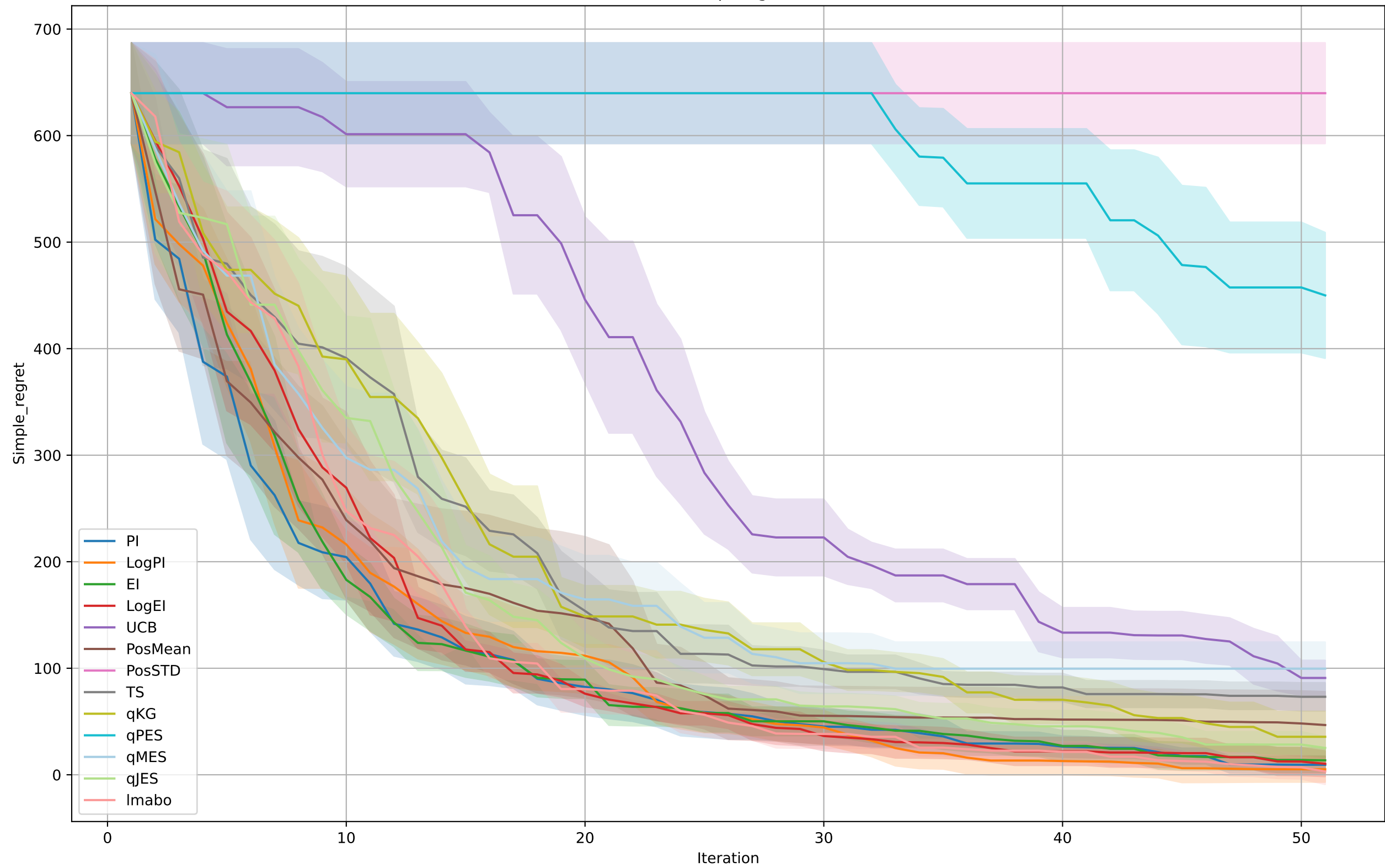
SharpRidge
