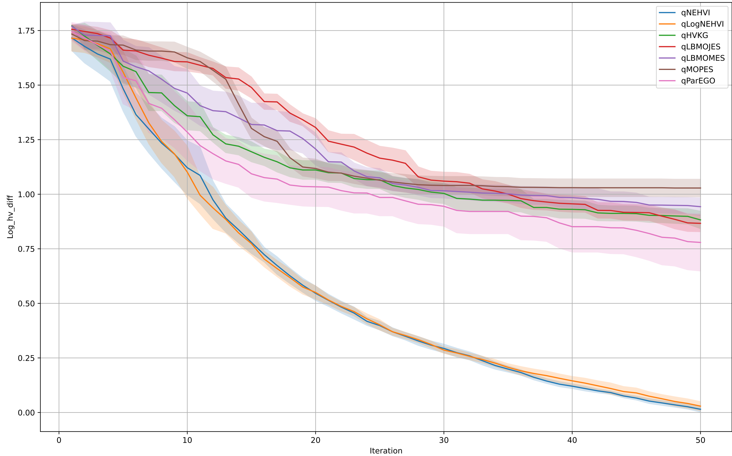
BraninCurrin
