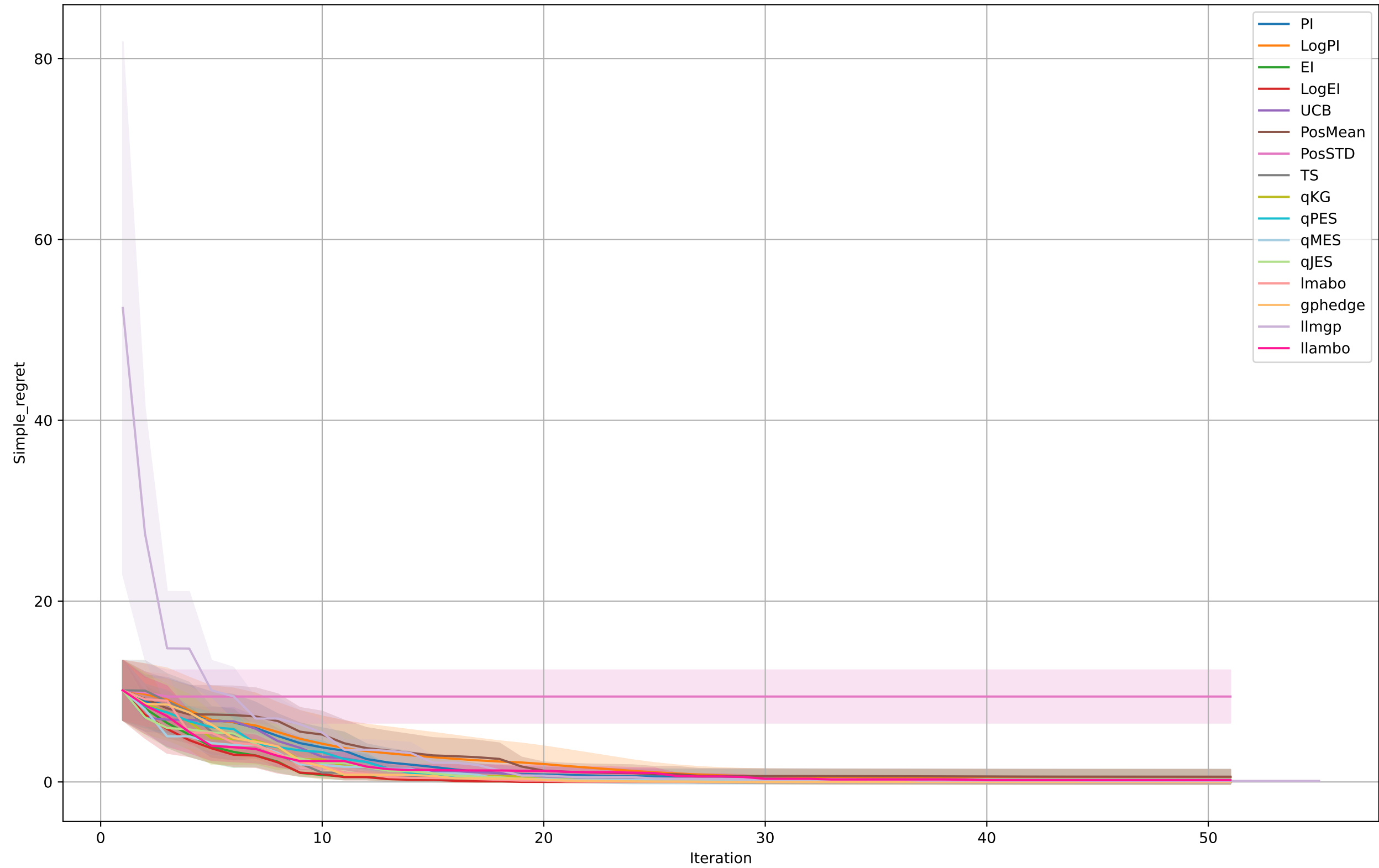
Branin
