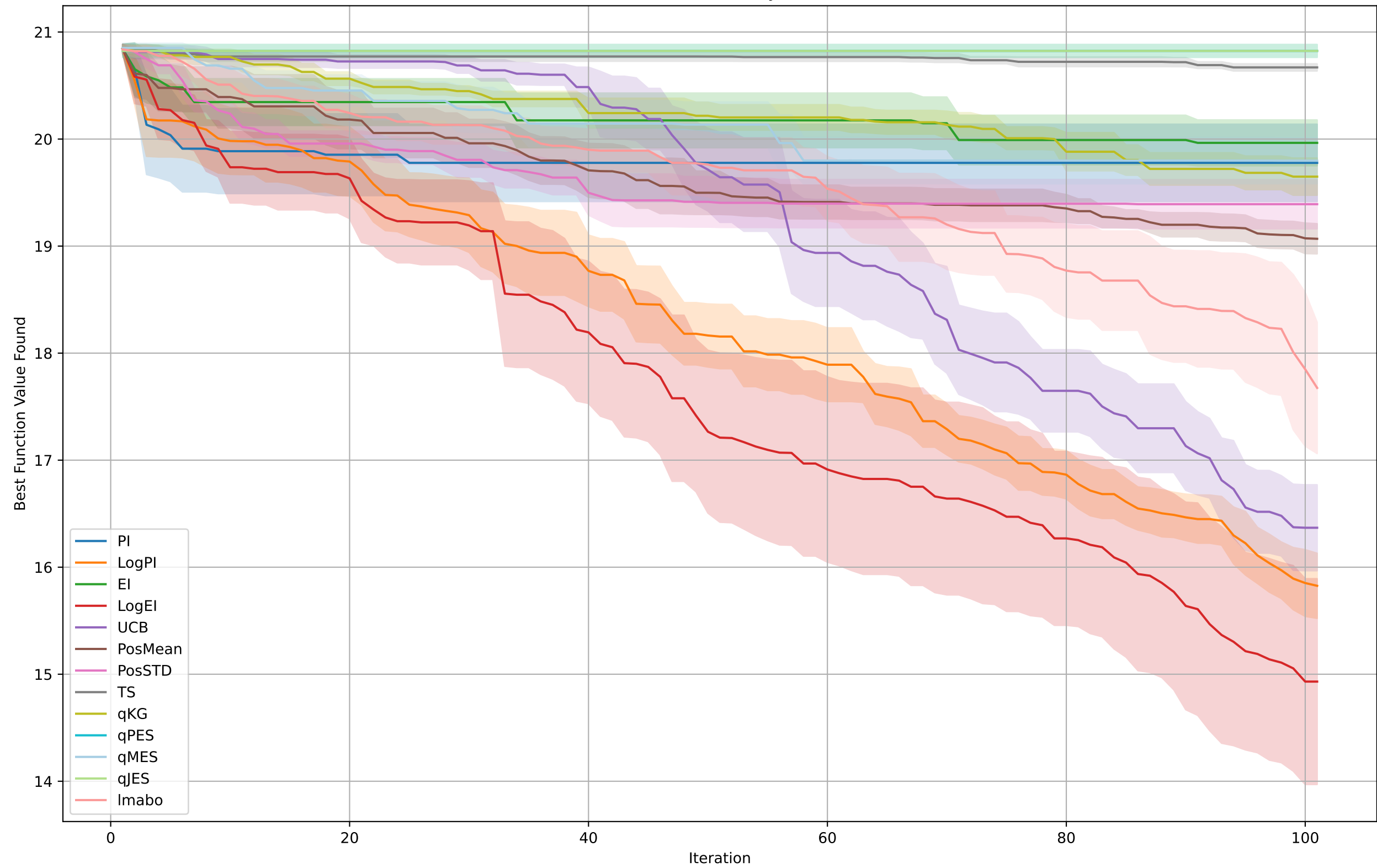
BO on Ackley
