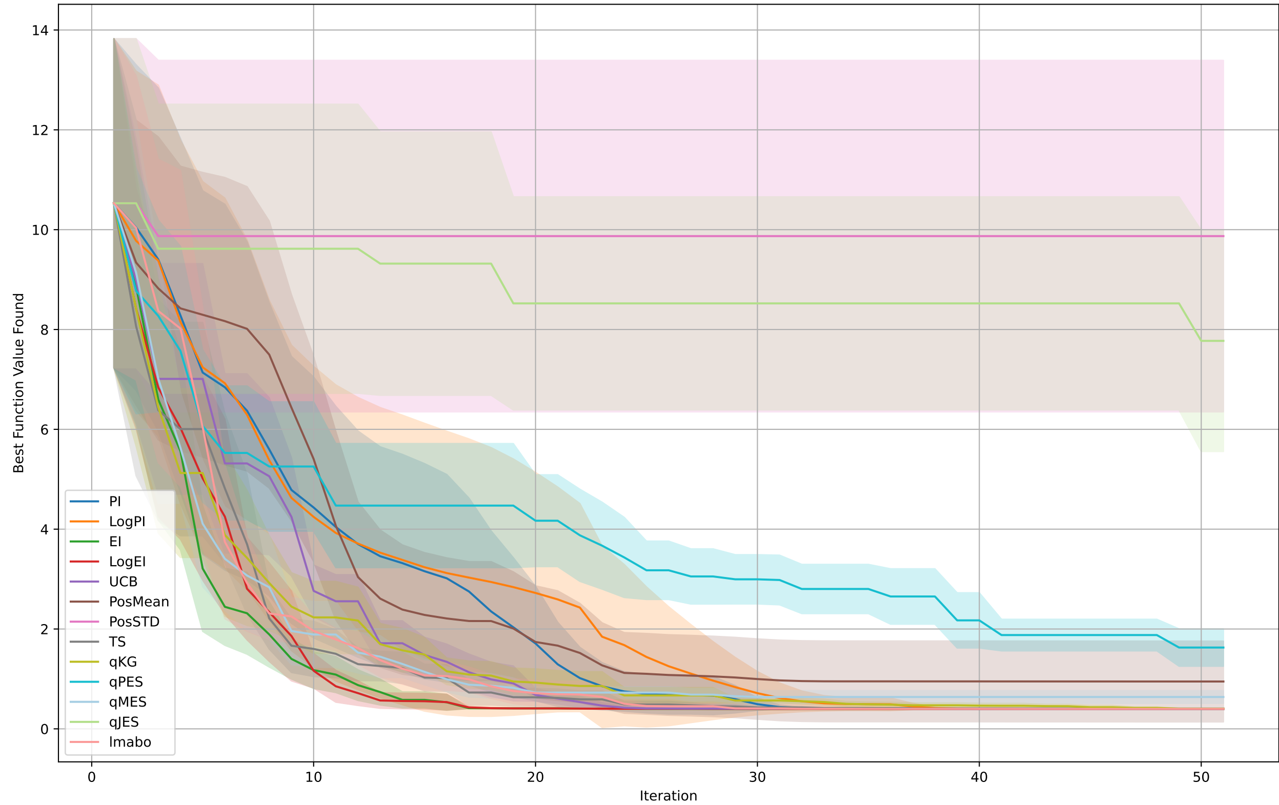
BO on Branin
