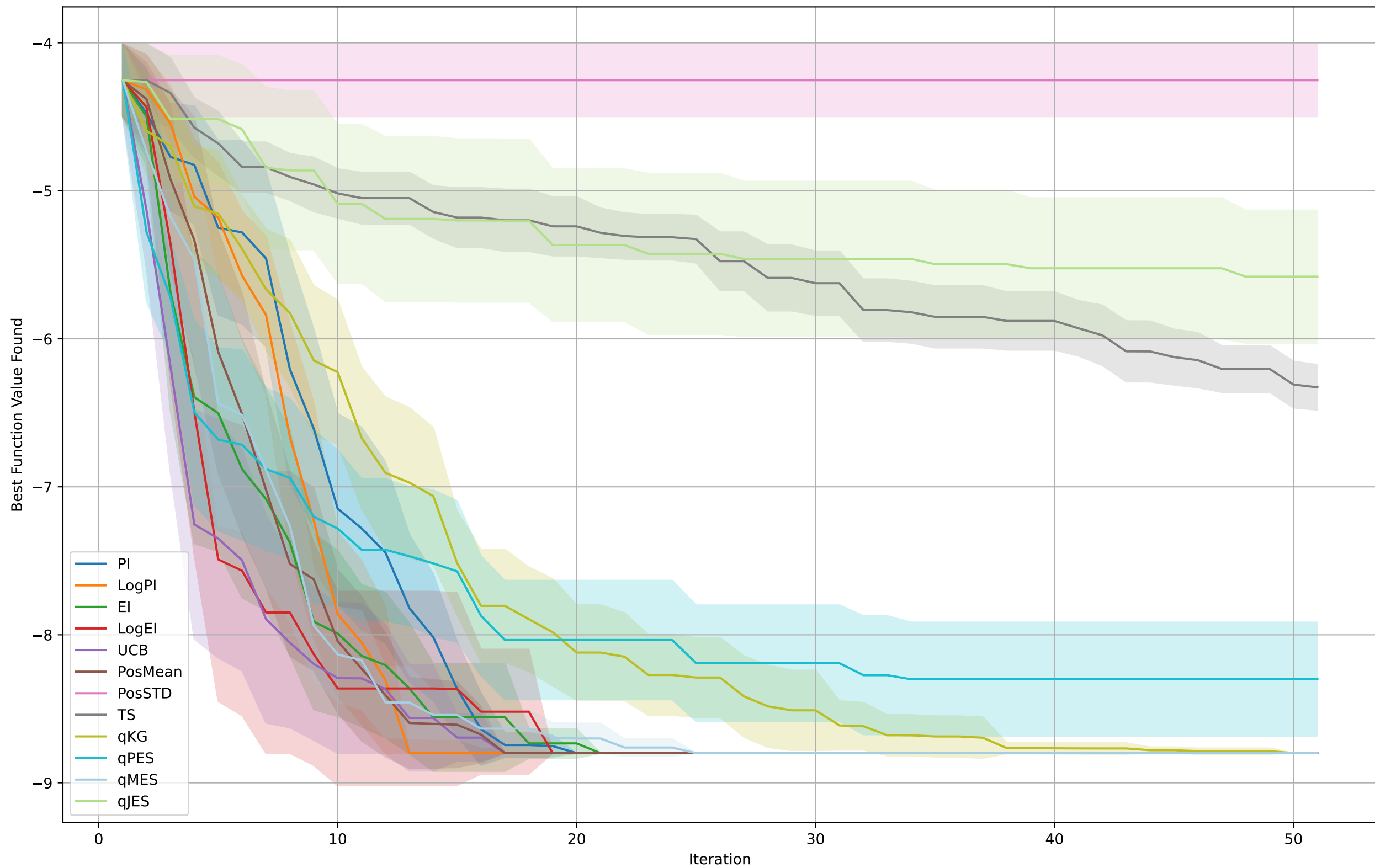
BO on Cosine8
