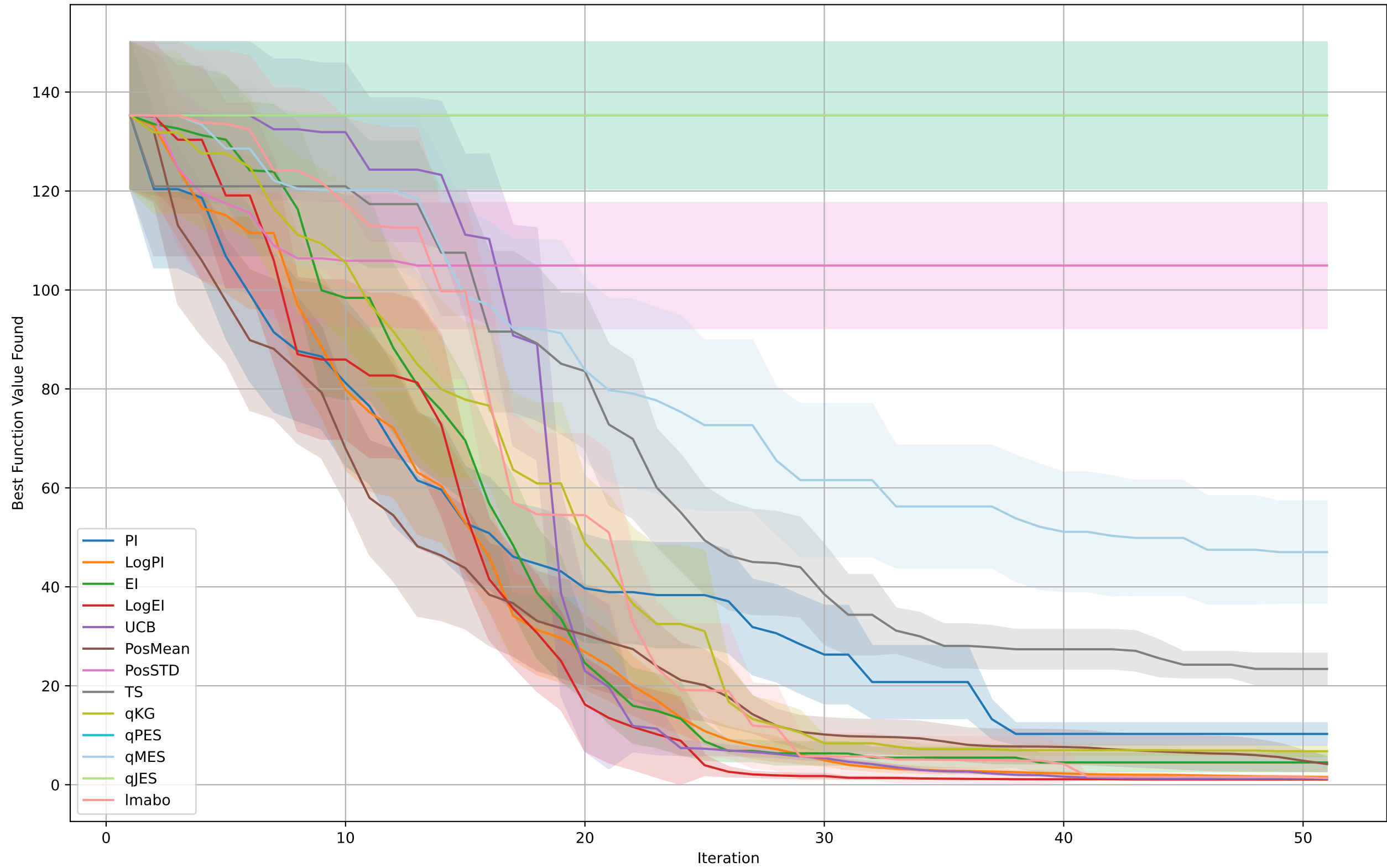
BO on Griewank
