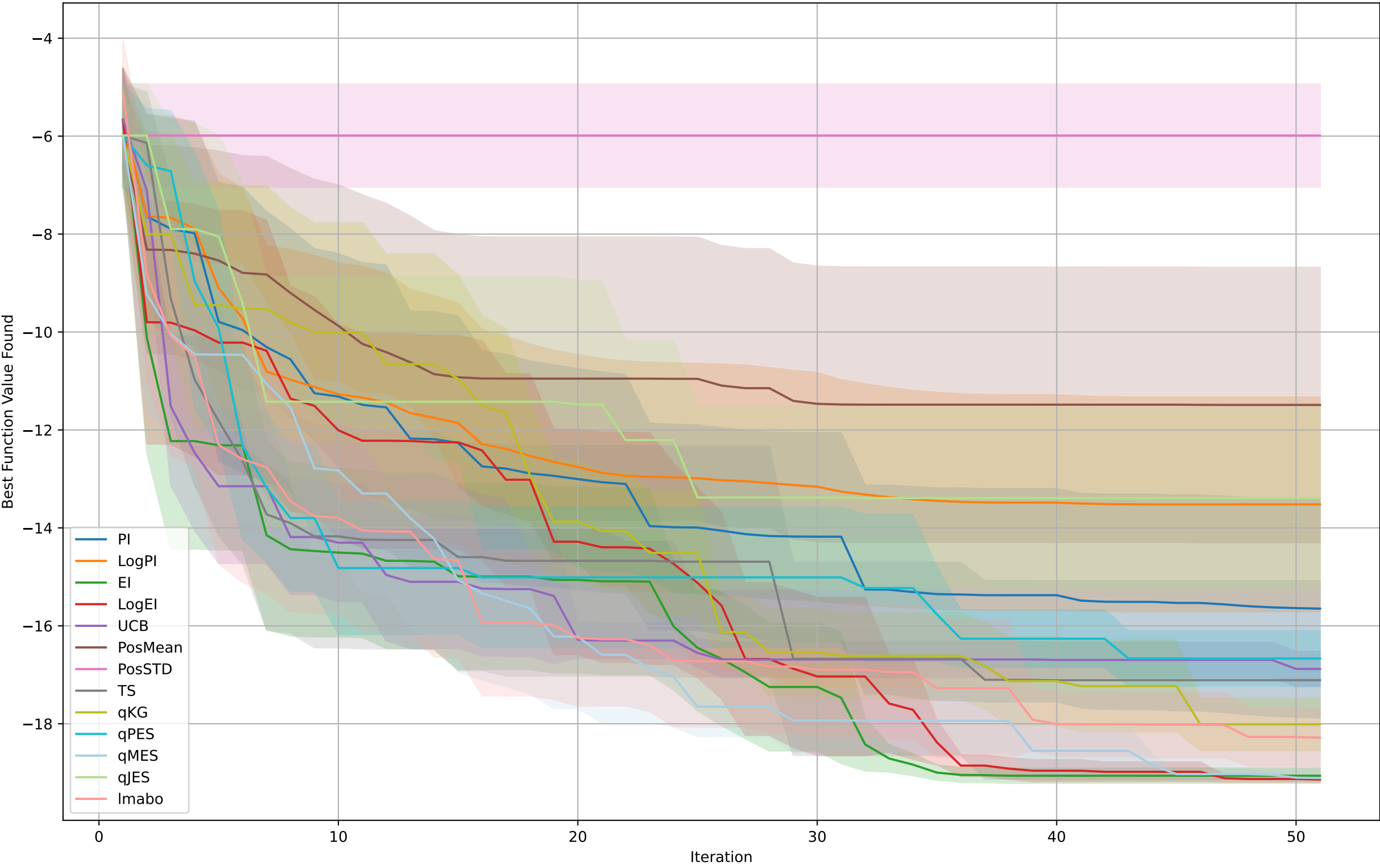
BO on HolderTable
