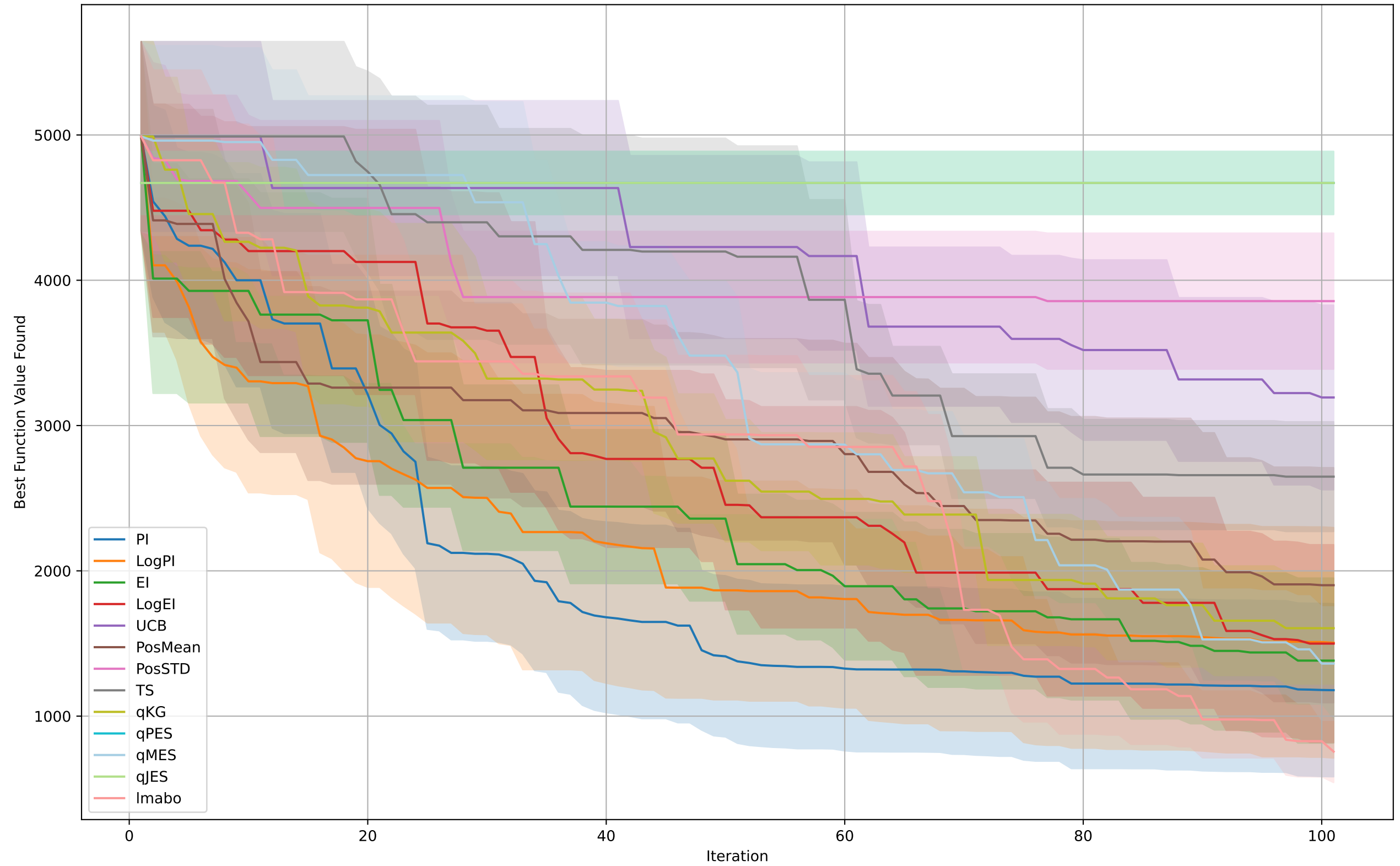
BO on Powell
