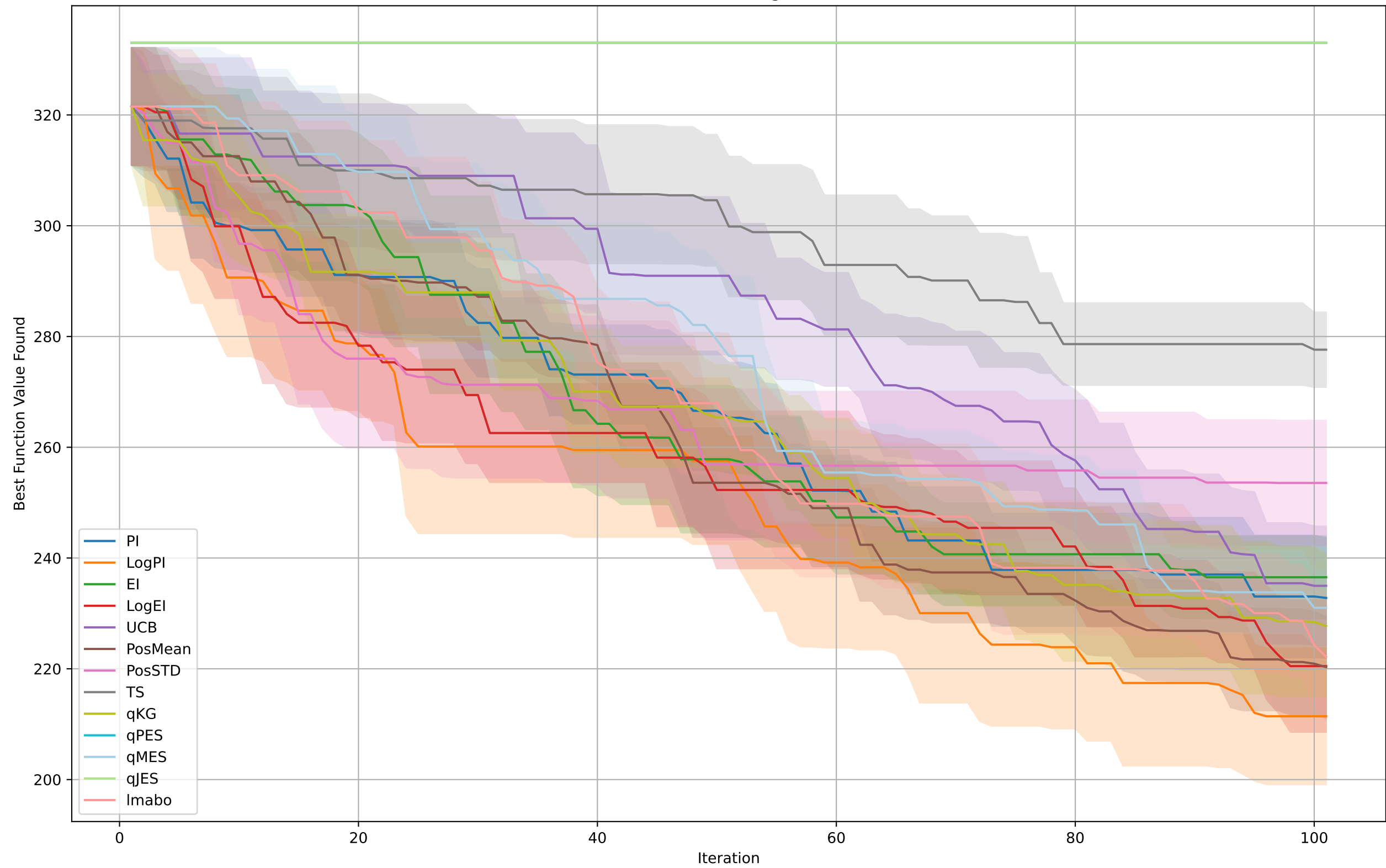
BO on Rastrigin
