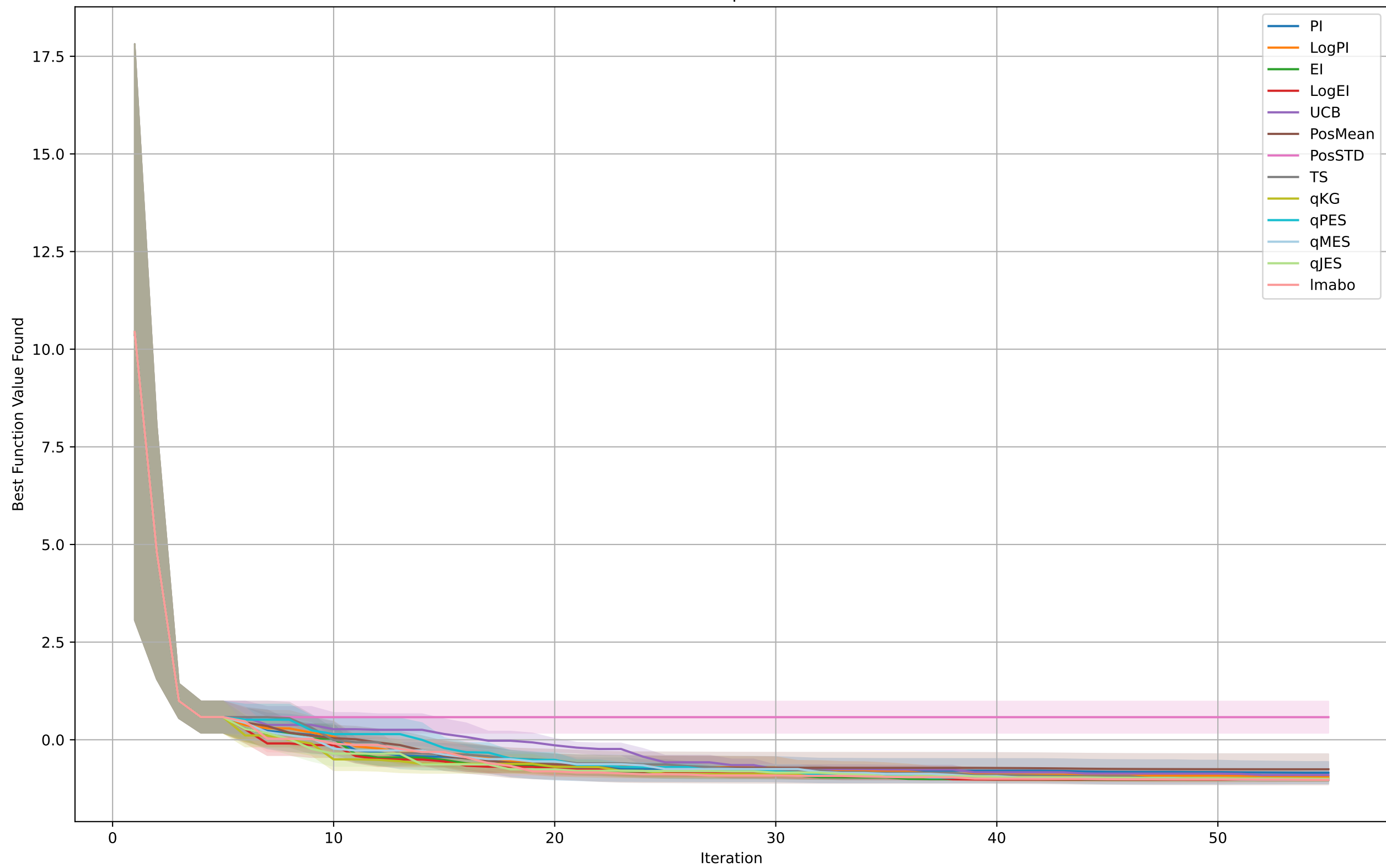
SixHumpCamel
