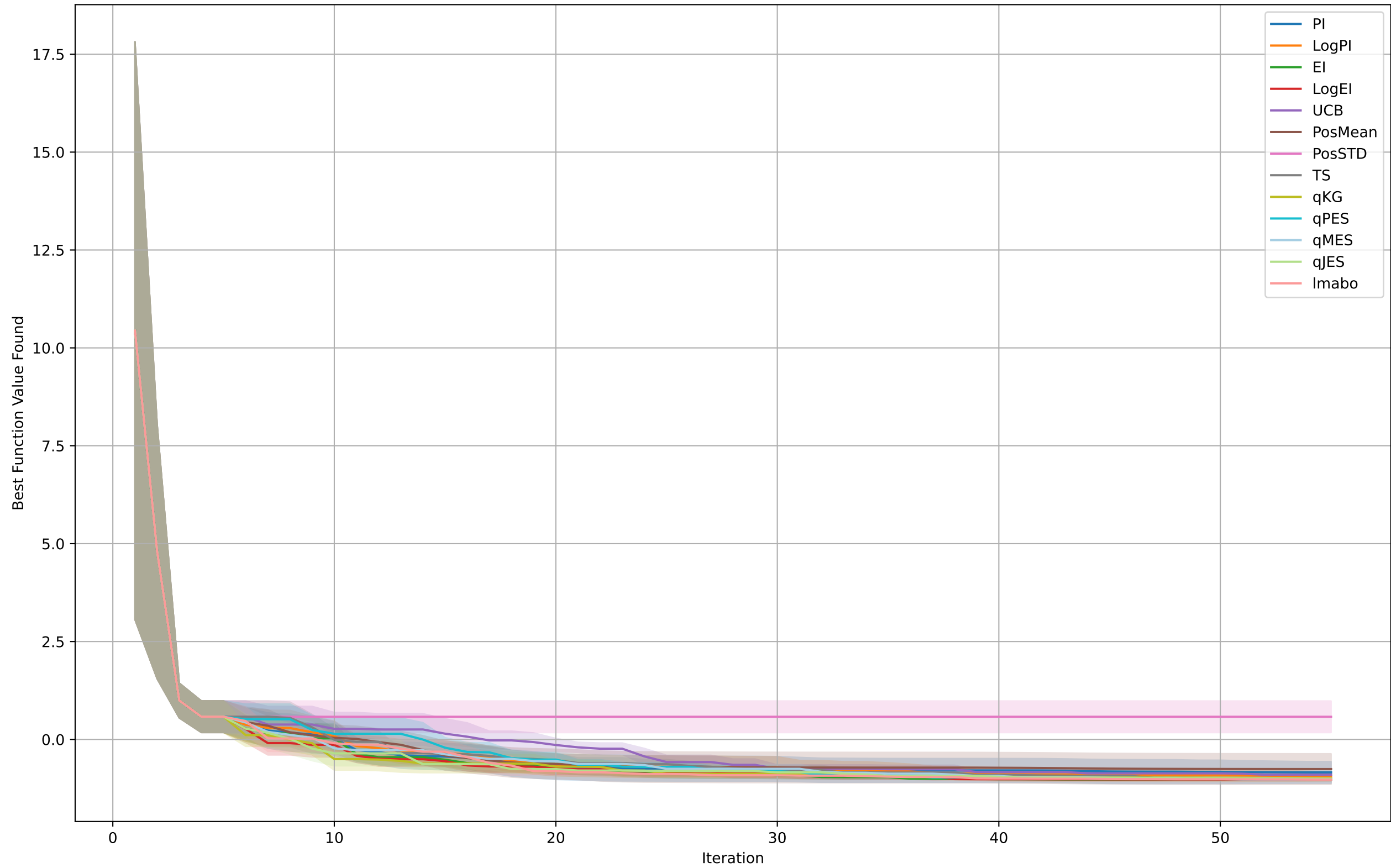
SixHumpCamel
