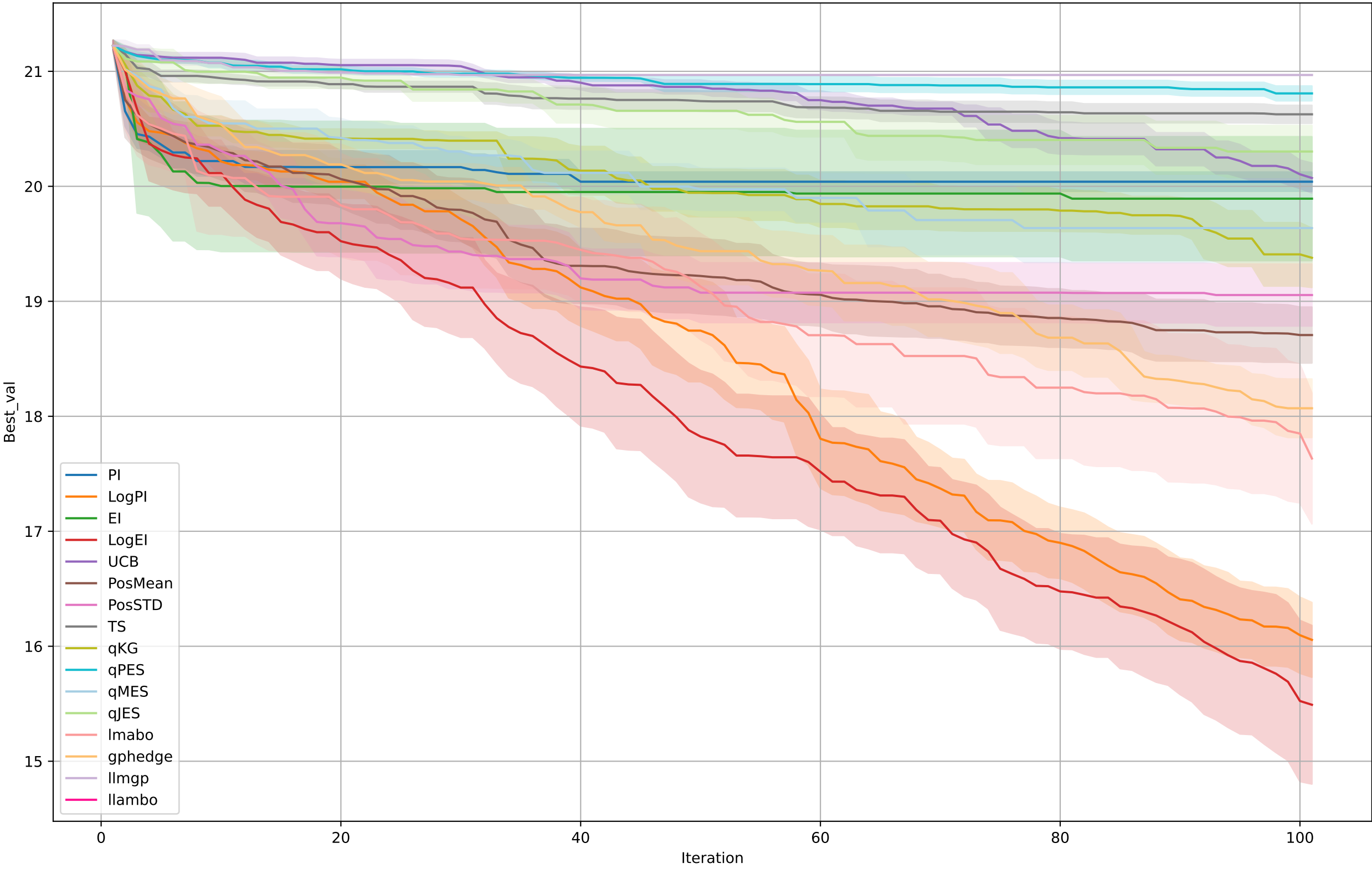
Ackley
