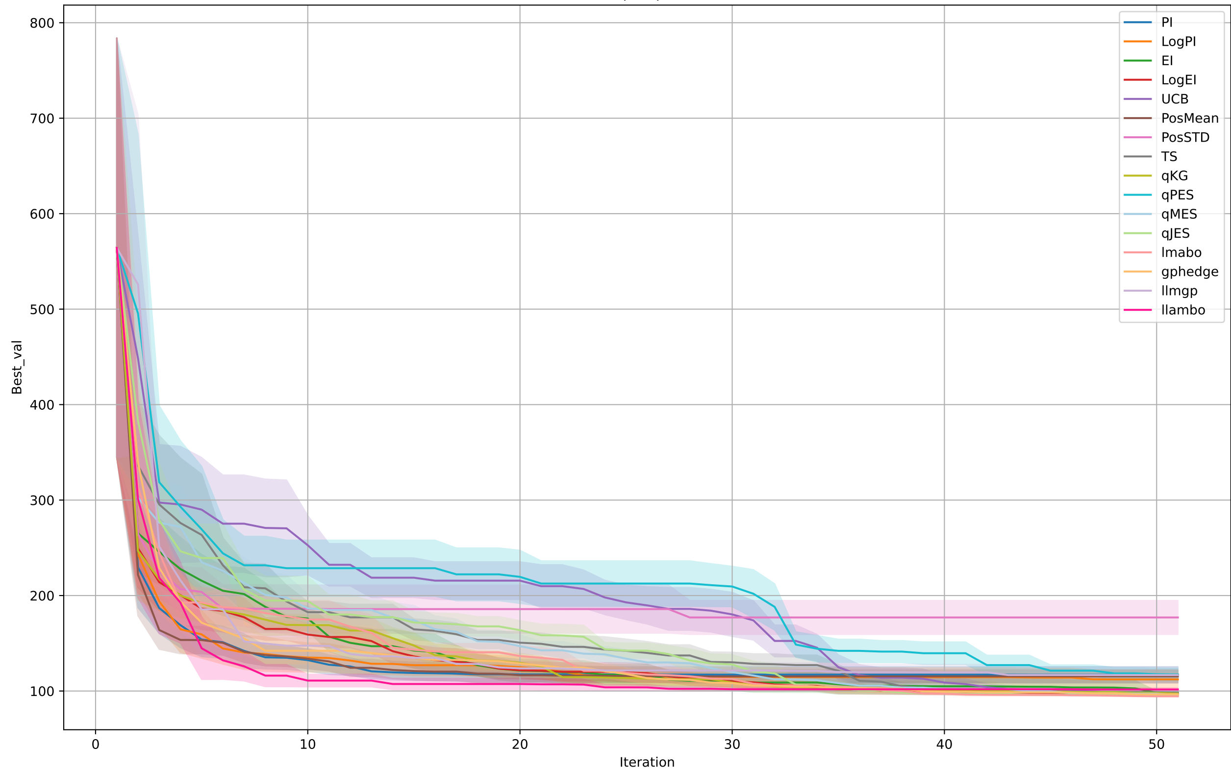
StepEllipsoid
