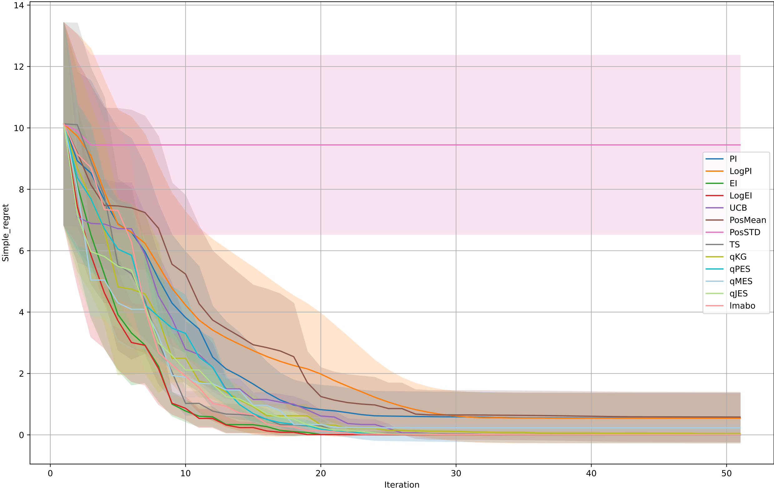
Branin
