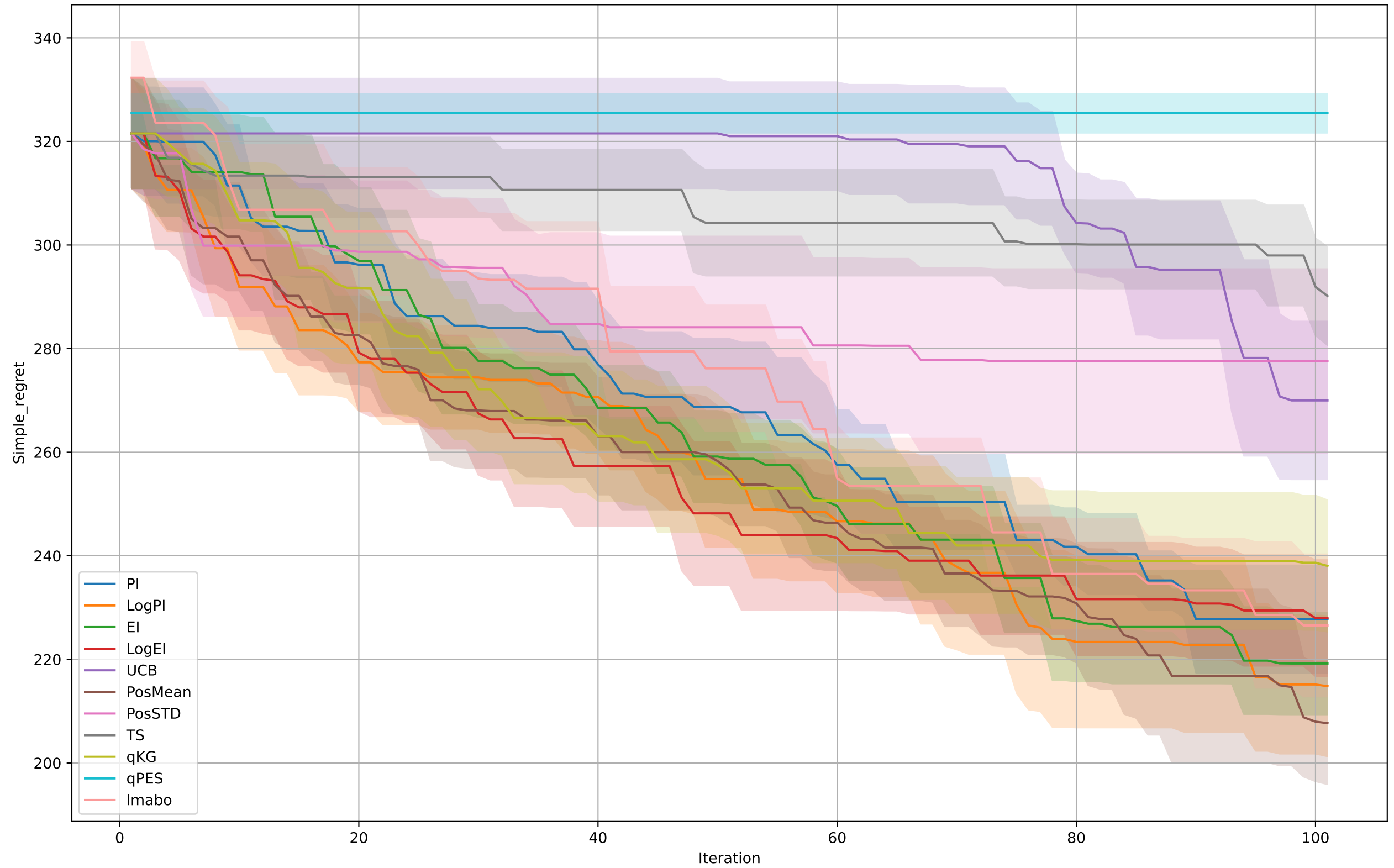
Rastrigin
