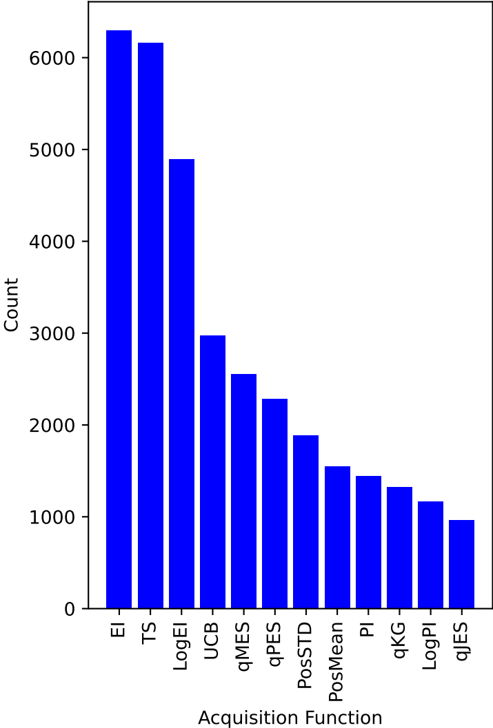
Acquisition Function Count Across All Problems
