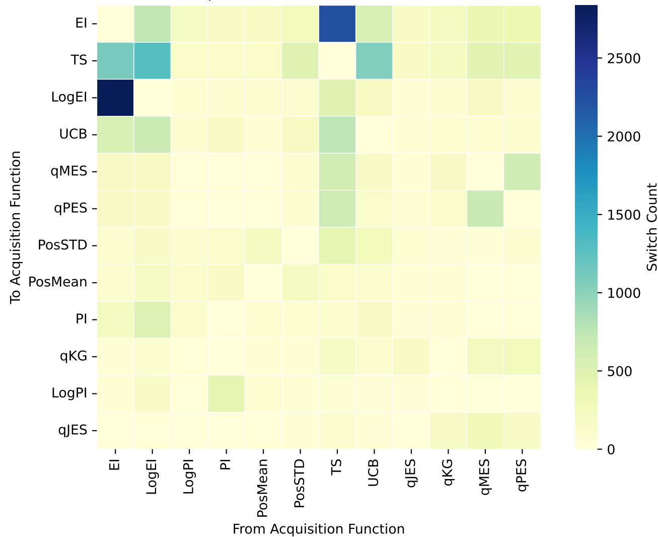
Acquisition Function Switch Count
