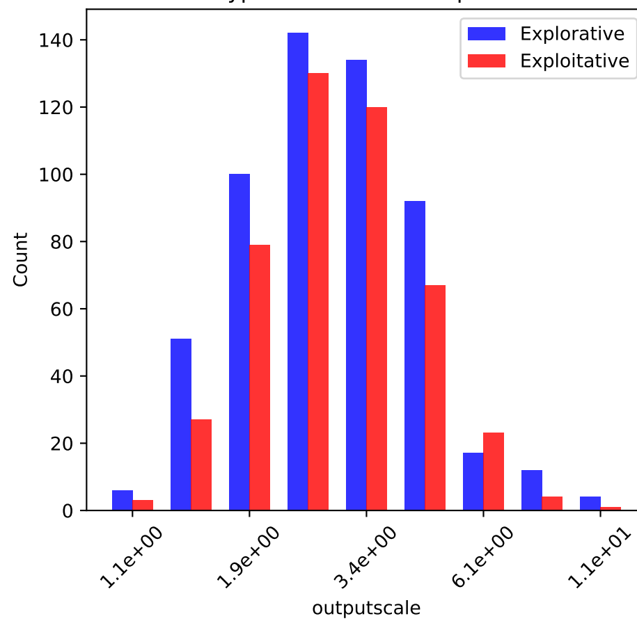
AF Type Distribution: outputscale
