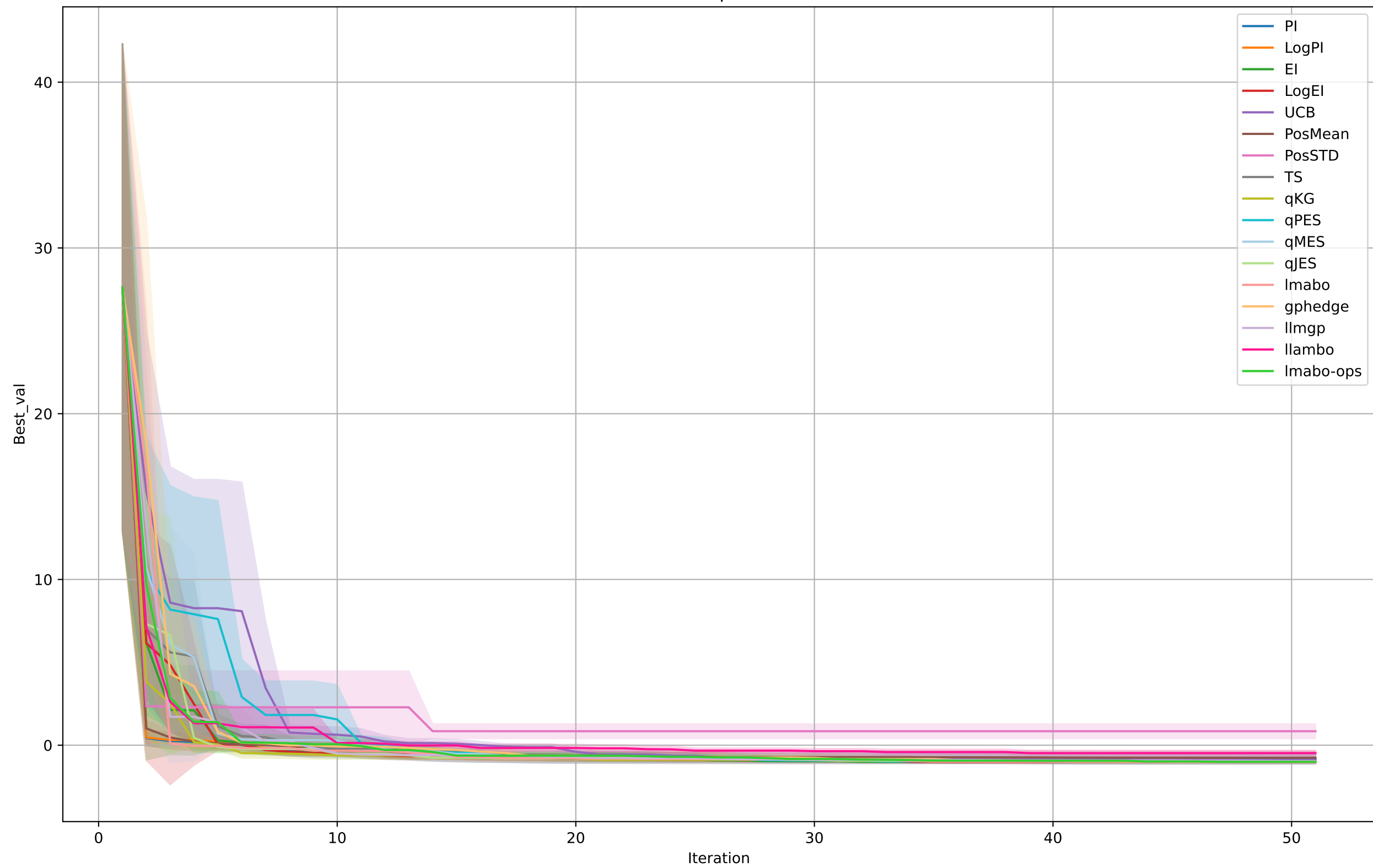
SixHumpCamel
