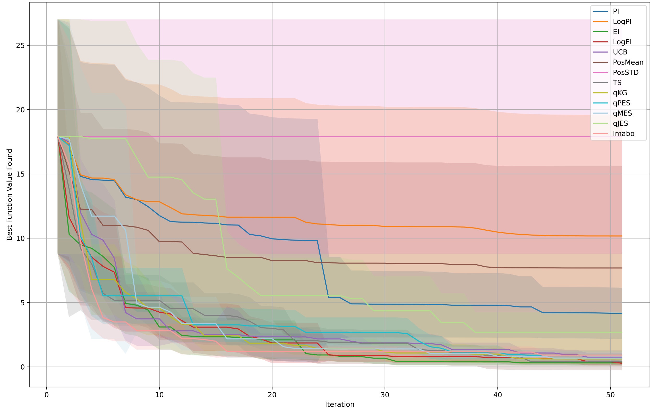
BO on Beale
