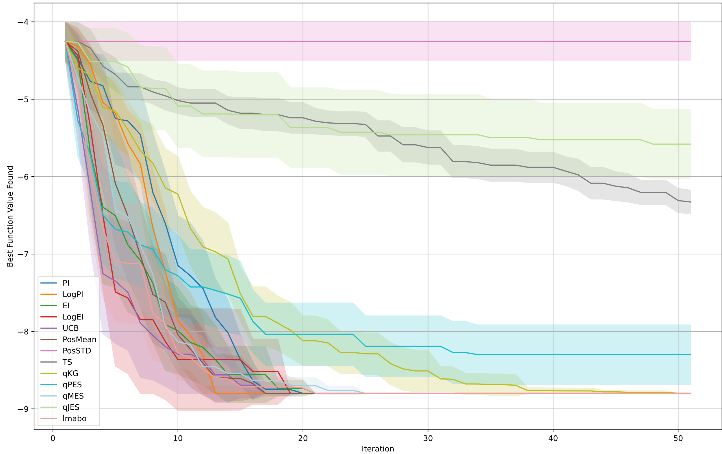
BO on Cosine8
