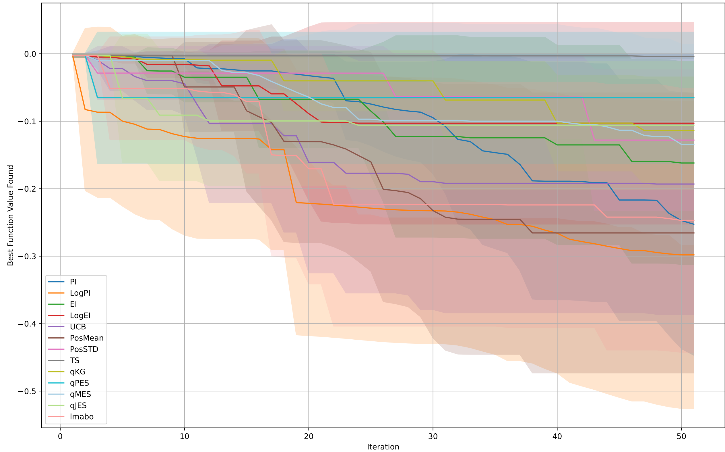
BO on Easom
