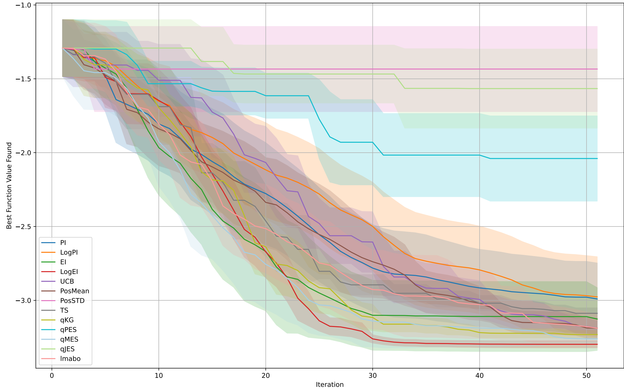
BO on Hartmann
