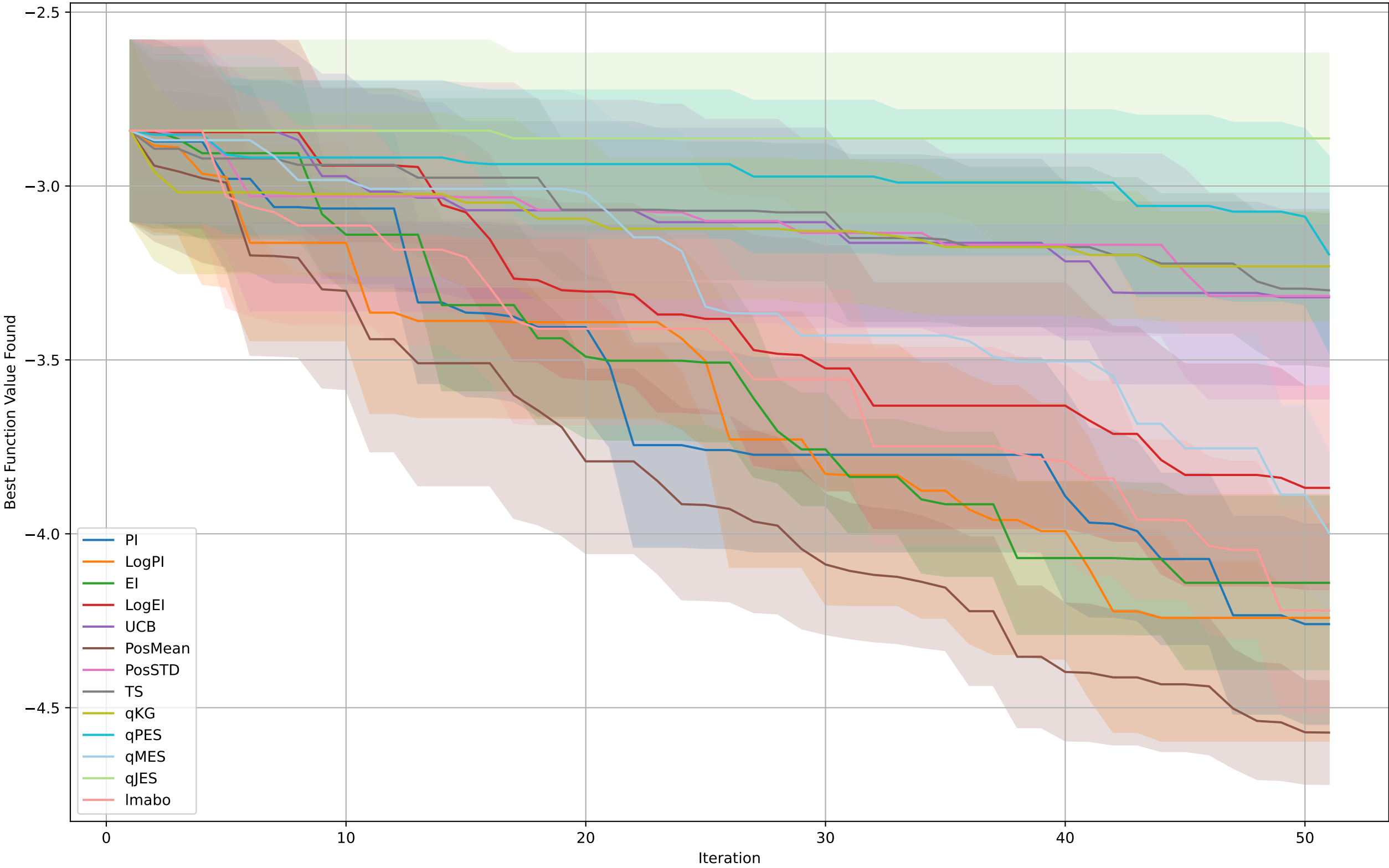
BO on Michalewicz
