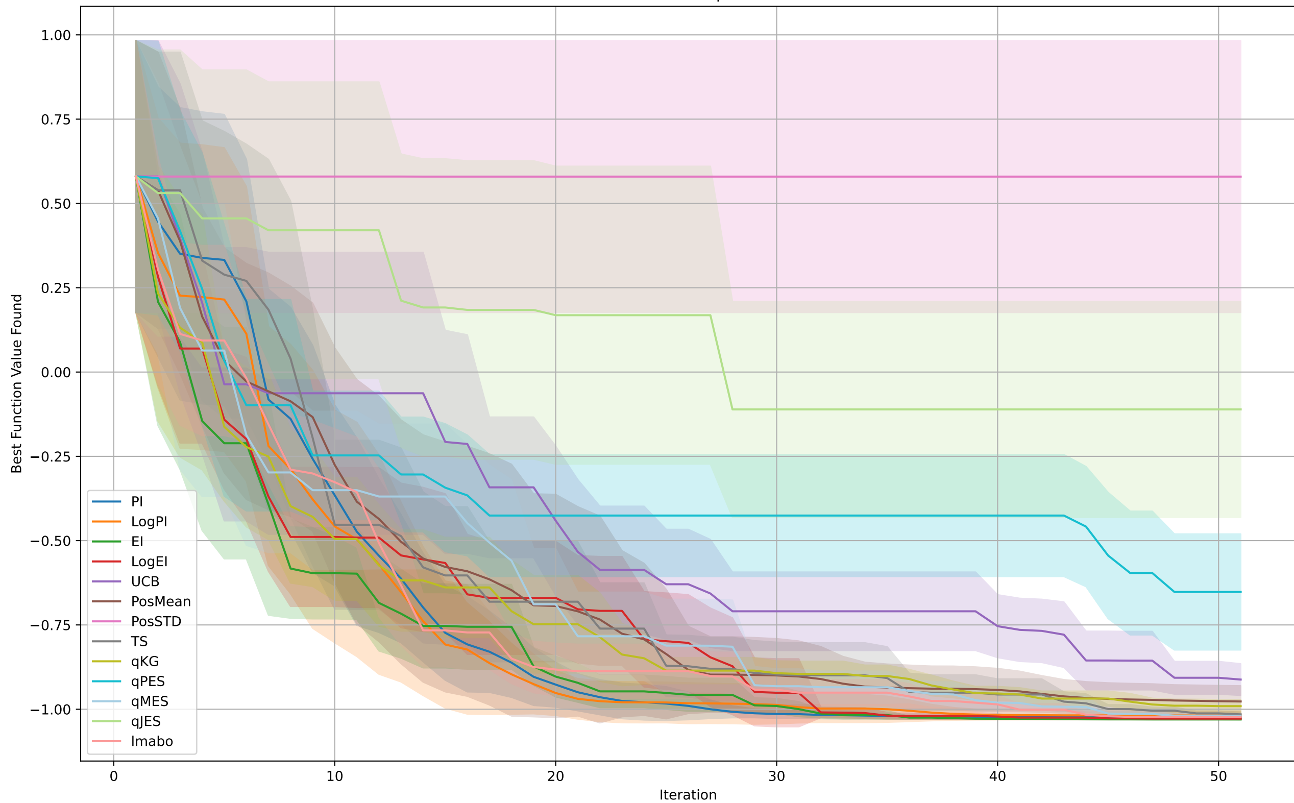
BO on SixHumpCamel
