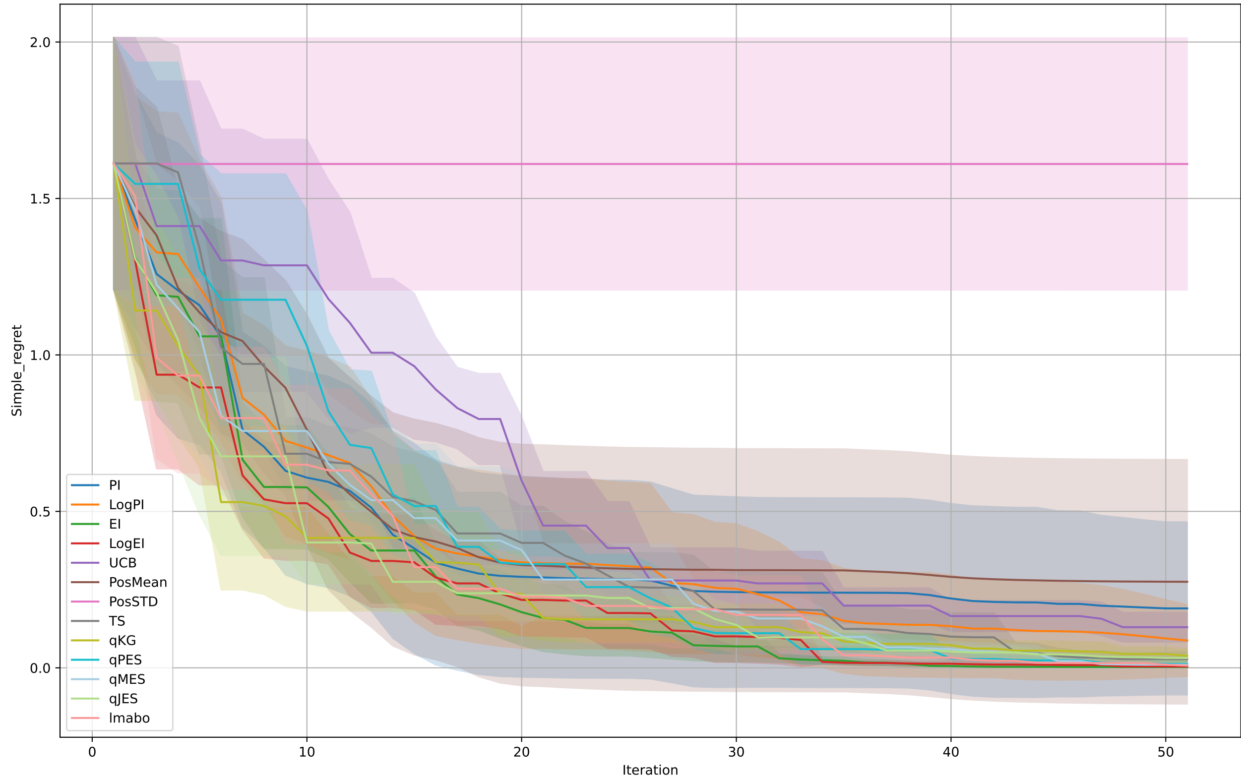
SixHumpCamel
